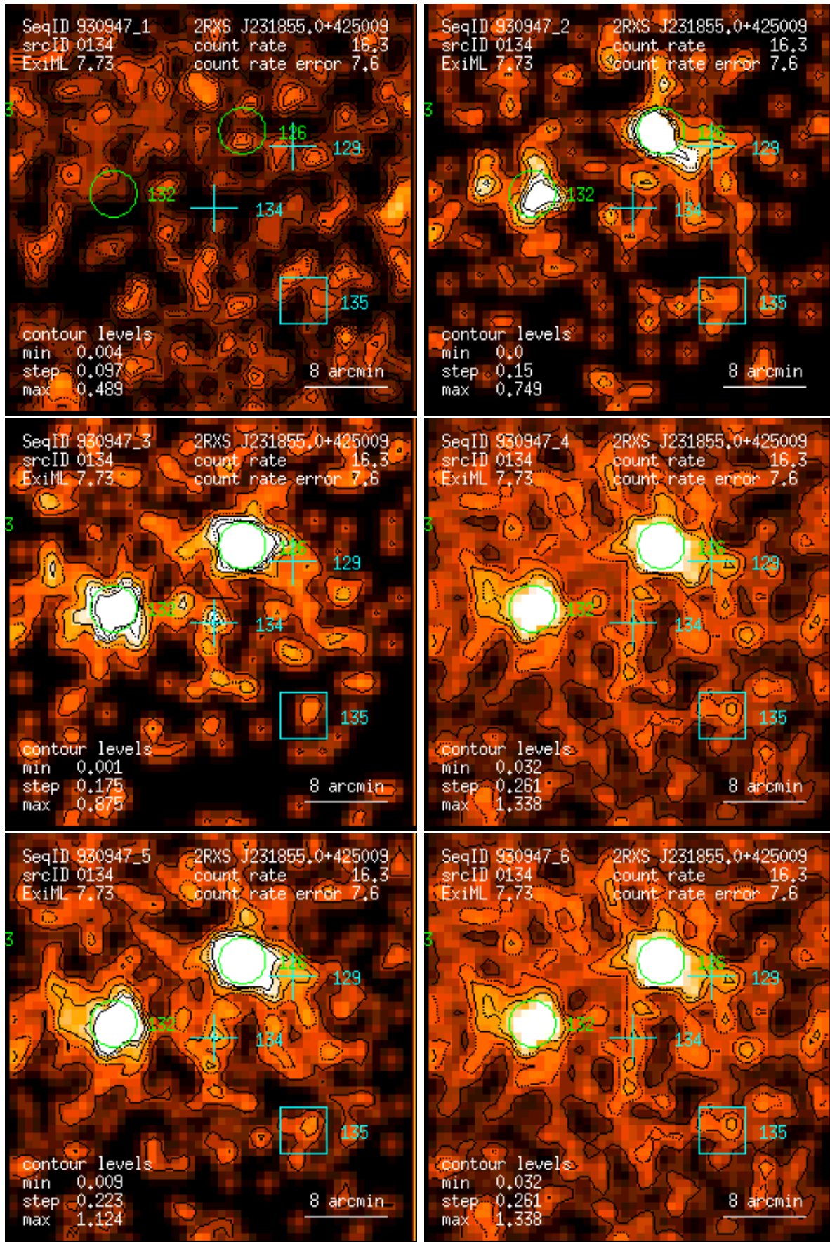
Figure 134: RASS 930947: detection 0134: band rate images, Gaussian filter: (1) PSPC channels 11 – 41, (2) 52 – 90, (3) 91 – 201, (4) 11 – 235, (5) 52 – 201, (6) 11 – 201. Broad band rates in counts/ks. Band rate contour levels in counts/ks/arcmin 2 .
