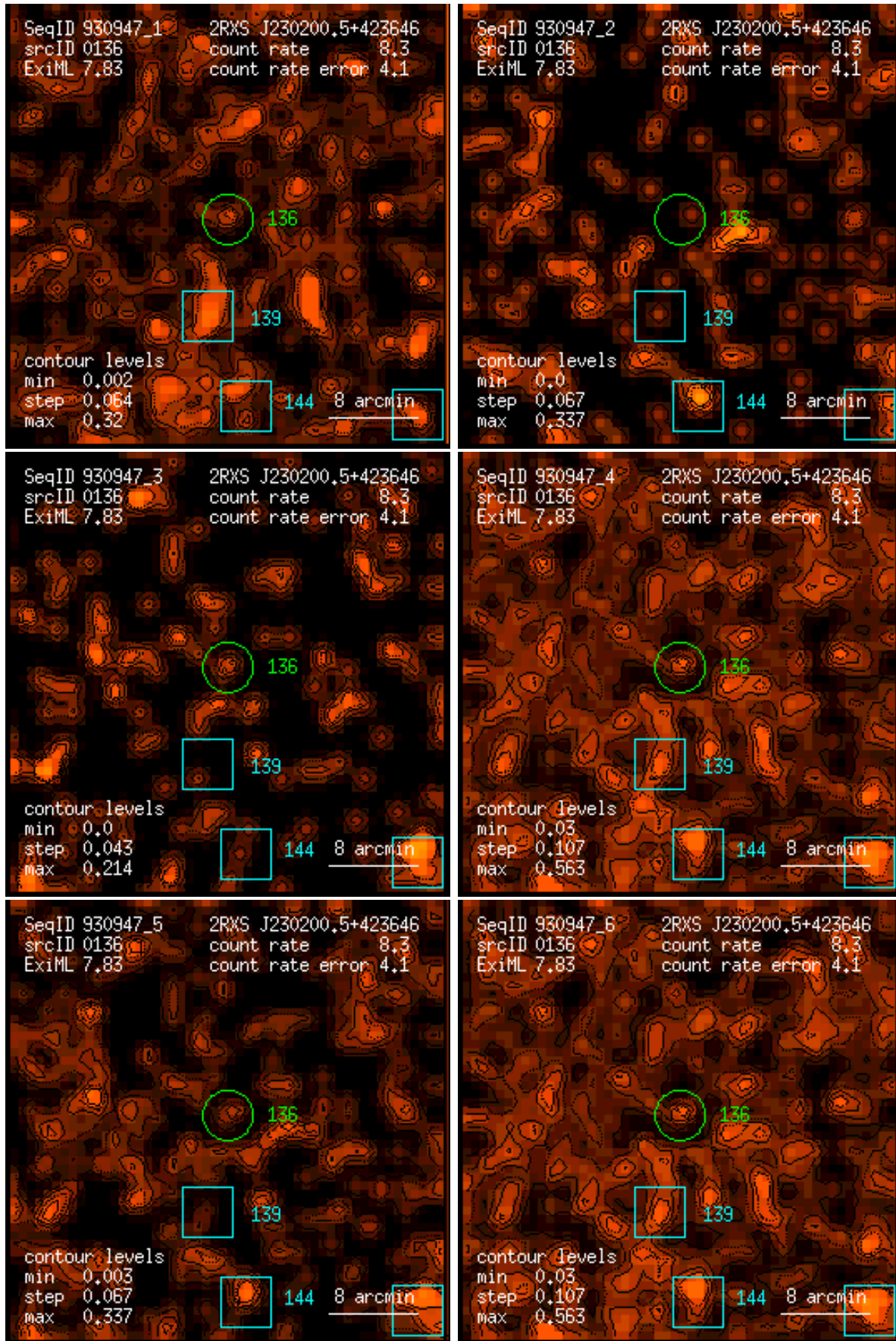
Figure 136: RASS 930947: detection 0136: band rate images, Gaussian filter: (1) PSPC channels 11 – 41, (2) 52 – 90, (3) 91 – 201, (4) 11 – 235, (5) 52 – 201, (6) 11 – 201. Broad band rates in counts/ks. Band rate contour levels in counts/ks/arcmin 2 .
