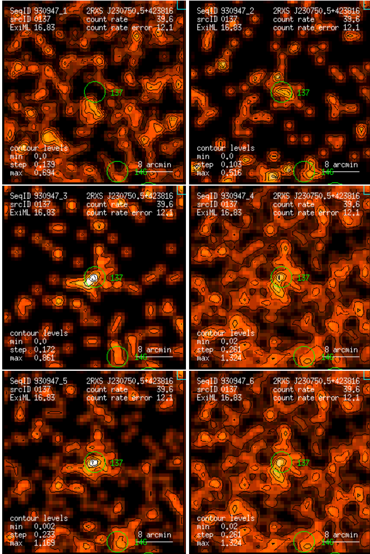
Figure 137: RASS 930947: detection 0137: band rate images, Gaussian filter: (1) PSPC channels 11 – 41, (2) 52 – 90, (3) 91 – 201, (4) 11 – 235, (5) 52 – 201, (6) 11 – 201. Broad band rates in counts/ks. Band rate contour levels in counts/ks/arcmin 2 .
