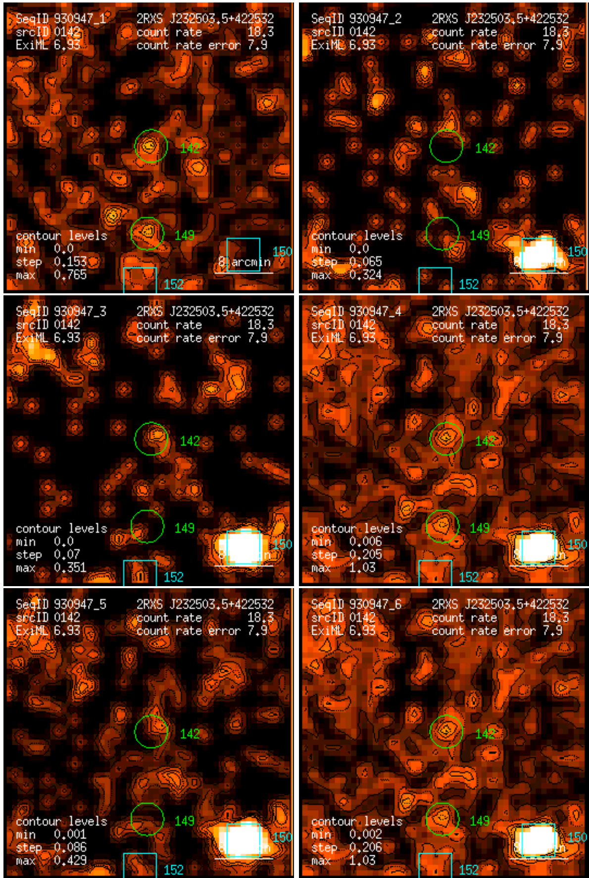
Figure 142: RASS 930947: detection 0142: band rate images, Gaussian filter: (1) PSPC channels 11 – 41, (2) 52 – 90, (3) 91 – 201, (4) 11 – 235, (5) 52 – 201, (6) 11 – 201. Broad band rates in counts/ks. Band rate contour levels in counts/ks/arcmin 2 .
