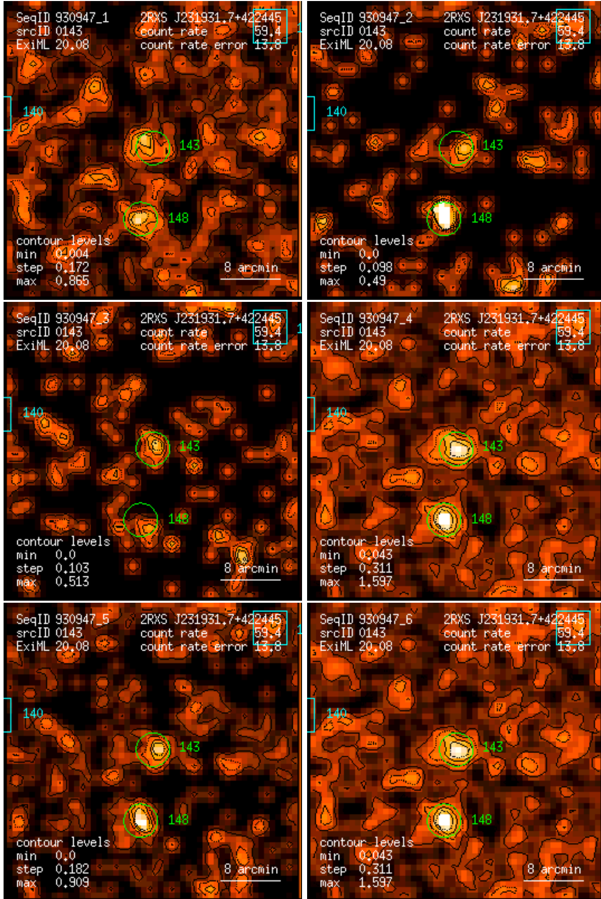
Figure 143: RASS 930947: detection 0143: band rate images, Gaussian filter: (1) PSPC channels 11 – 41, (2) 52 – 90, (3) 91 – 201, (4) 11 – 235, (5) 52 – 201, (6) 11 – 201. Broad band rates in counts/ks. Band rate contour levels in counts/ks/arcmin 2 .
