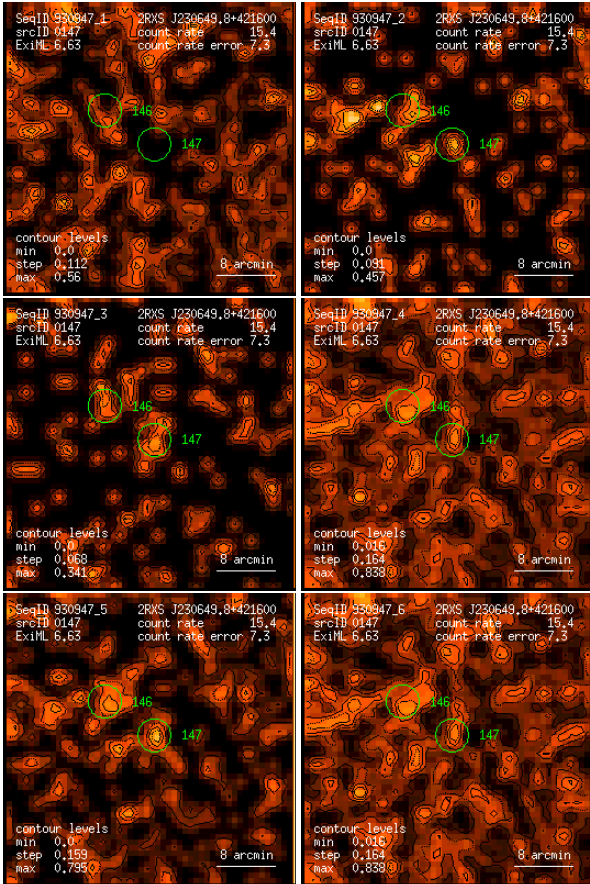
Figure 147: RASS 930947: detection 0147: band rate images, Gaussian filter: (1) PSPC channels 11 – 41, (2) 52 – 90, (3) 91 – 201, (4) 11 – 235, (5) 52 – 201, (6) 11 – 201. Broad band rates in counts/ks. Band rate contour levels in counts/ks/arcmin 2 .
