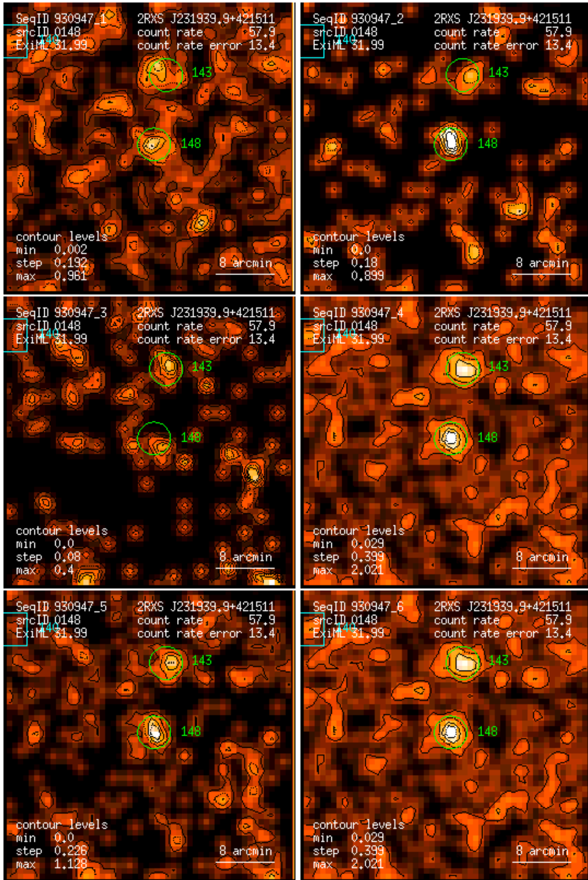
Figure 148: RASS 930947: detection 0148: band rate images, Gaussian filter: (1) PSPC channels 11 – 41, (2) 52 – 90, (3) 91 – 201, (4) 11 – 235, (5) 52 – 201, (6) 11 – 201. Broad band rates in counts/ks. Band rate contour levels in counts/ks/arcmin 2 .
