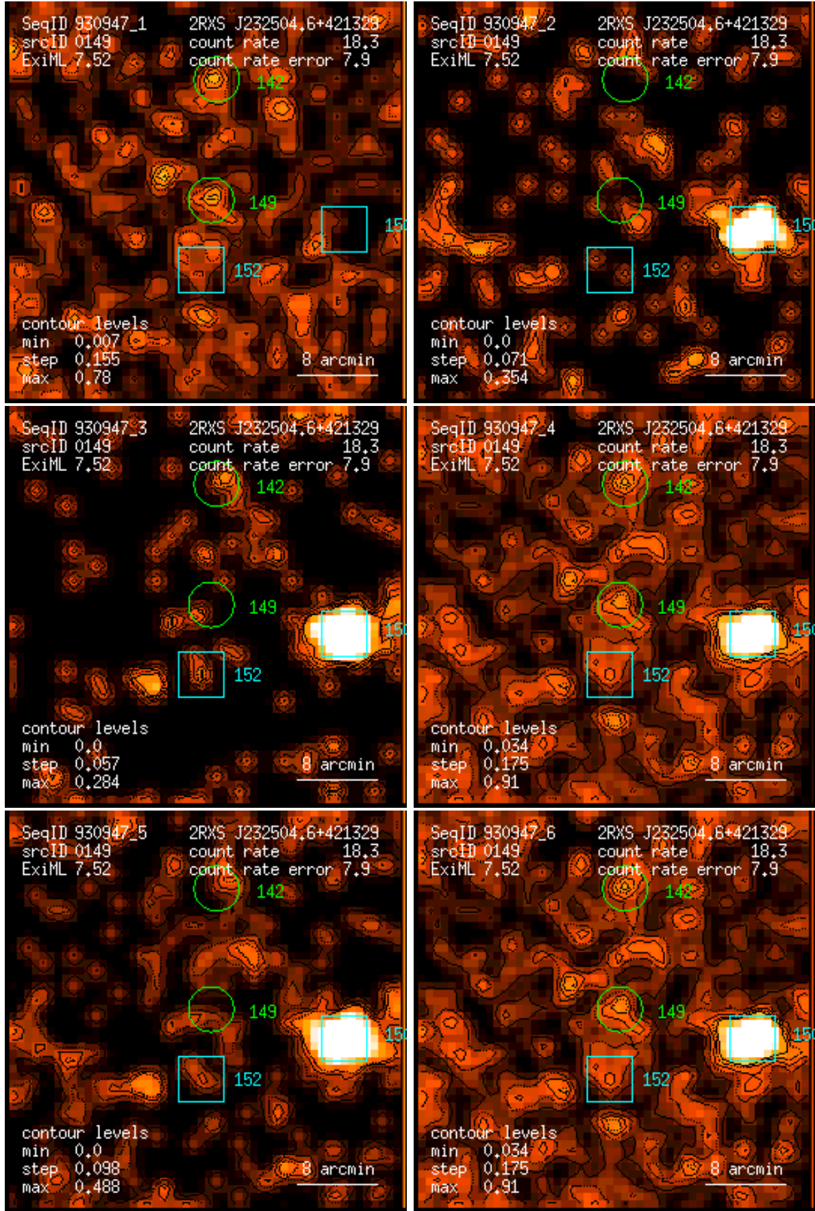
Figure 149: RASS 930947: detection 0149: band rate images, Gaussian filter: (1) PSPC channels 11 – 41, (2) 52 – 90, (3) 91 – 201, (4) 11 – 235, (5) 52 – 201, (6) 11 – 201. Broad band rates in counts/ks. Band rate contour levels in counts/ks/arcmin 2 .
