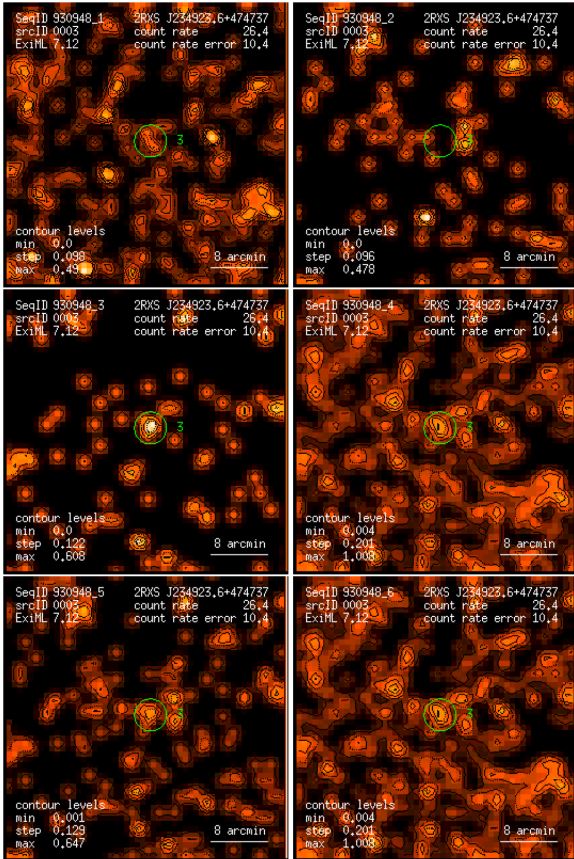
Figure 3: RASS 930948: detection 0003: band rate images, Gaussian filter: (1) PSPC channels 11 – 41, (2) 52 – 90, (3) 91 – 201, (4) 11 – 235, (5) 52 – 201, (6) 11 – 201. Broad band rates in counts/ks. Band rate contour levels in counts/ks/arcmin 2 .
