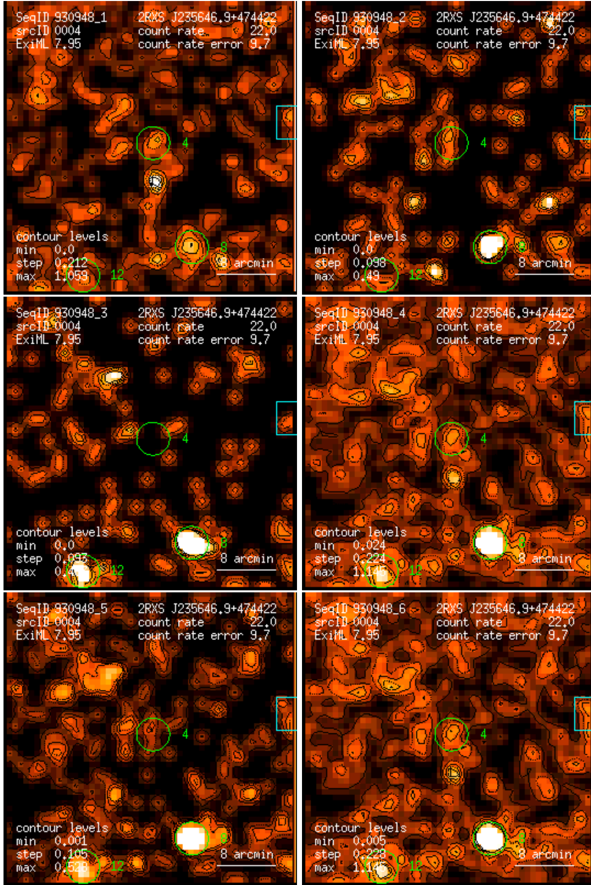
Figure 4: RASS 930948: detection 0004: band rate images, Gaussian filter: (1) PSPC channels 11 – 41, (2) 52 – 90, (3) 91 – 201, (4) 11 – 235, (5) 52 – 201, (6) 11 – 201. Broad band rates in counts/ks. Band rate contour levels in counts/ks/arcmin 2 .
