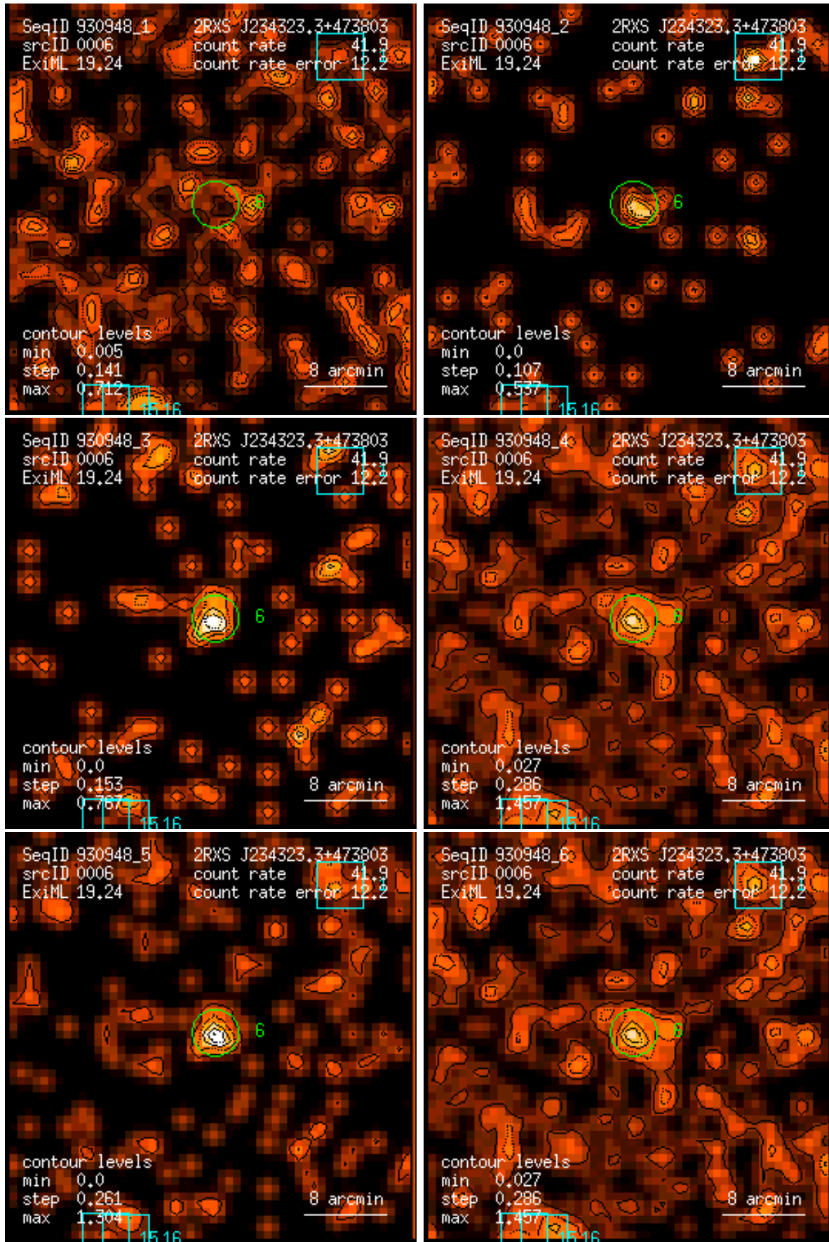
Figure 6: RASS 930948: detection 0006: band rate images, Gaussian filter: (1) PSPC channels 11 – 41, (2) 52 – 90, (3) 91 – 201, (4) 11 – 235, (5) 52 – 201, (6) 11 – 201. Broad band rates in counts/ks. Band rate contour levels in counts/ks/arcmin 2 .
