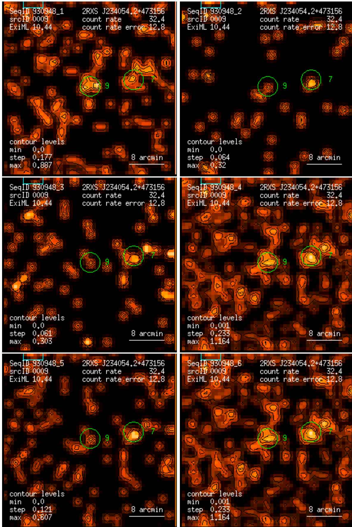
Figure 9: RASS 930948: detection 0009: band rate images, Gaussian filter: (1) PSPC channels 11 – 41, (2) 52 – 90, (3) 91 – 201, (4) 11 – 235, (5) 52 – 201, (6) 11 – 201. Broad band rates in counts/ks. Band rate contour levels in counts/ks/arcmin 2 .
