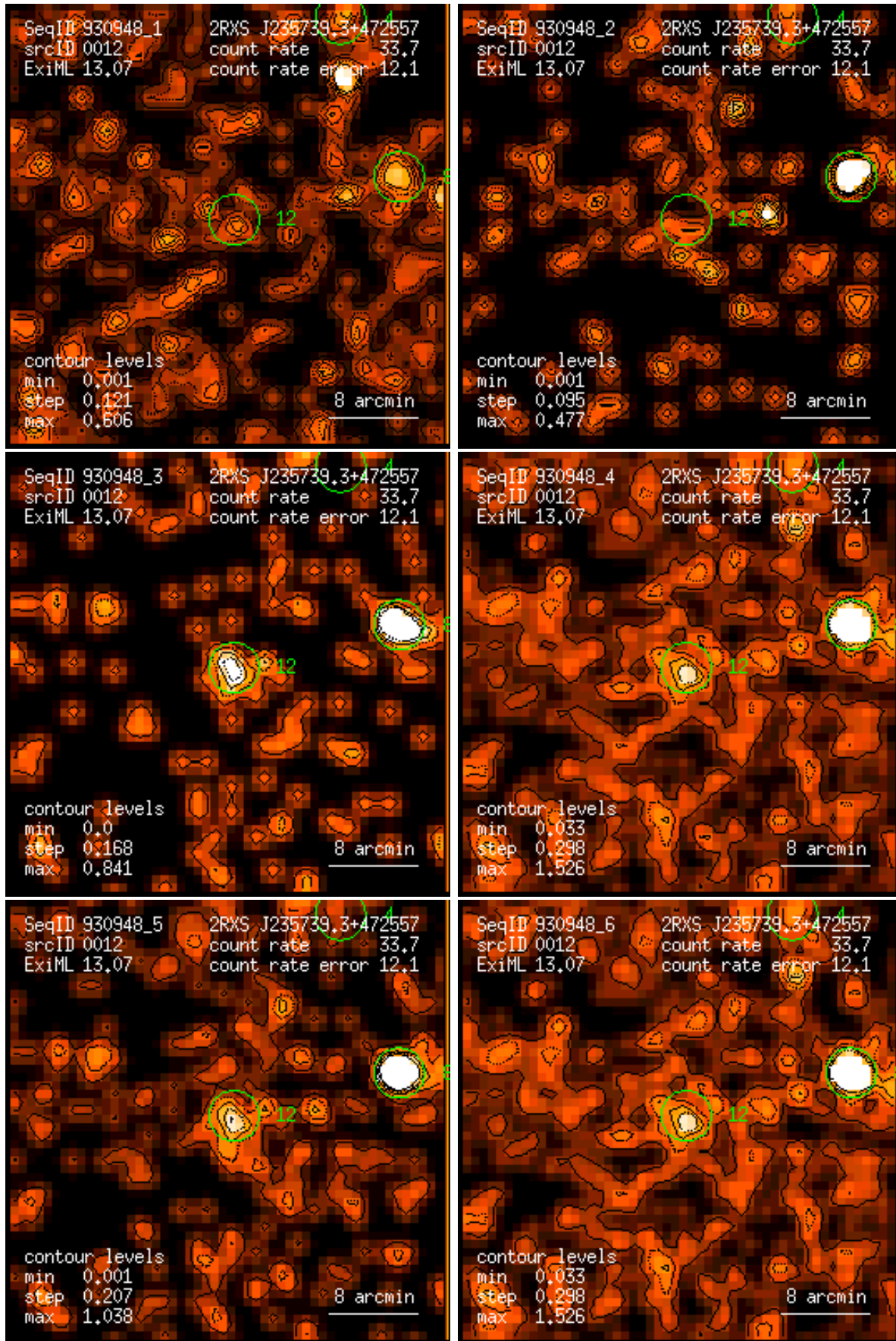
Figure 12: RASS 930948: detection 0012: band rate images, Gaussian filter: (1) PSPC channels 11 – 41, (2) 52 – 90, (3) 91 – 201, (4) 11 – 235, (5) 52 – 201, (6) 11 – 201. Broad band rates in counts/ks. Band rate contour levels in counts/ks/arcmin 2 .
