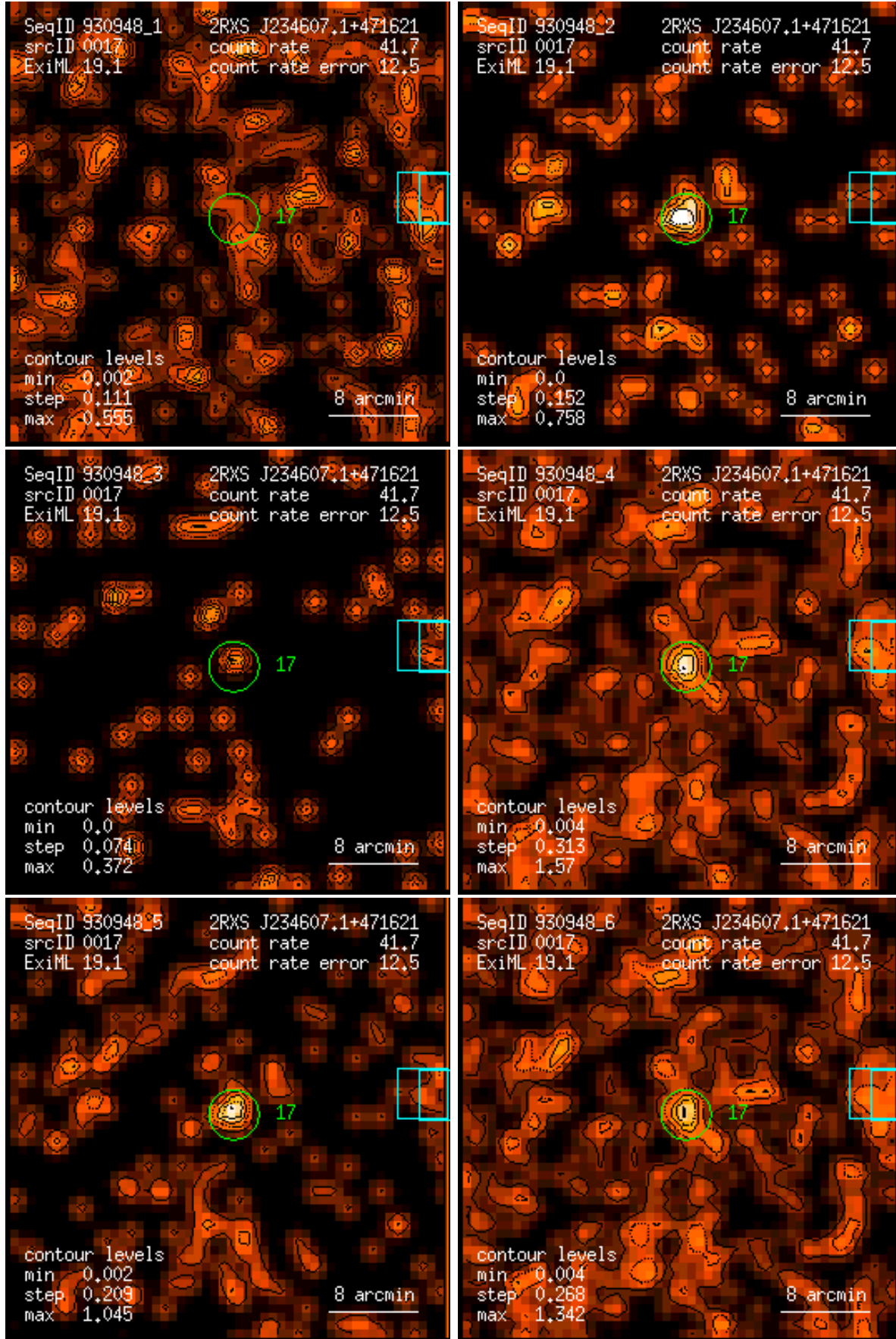
Figure 17: RASS 930948: detection 0017: band rate images, Gaussian filter: (1) PSPC channels 11 – 41, (2) 52 – 90, (3) 91 – 201, (4) 11 – 235, (5) 52 – 201, (6) 11 – 201. Broad band rates in counts/ks. Band rate contour levels in counts/ks/arcmin 2 .
