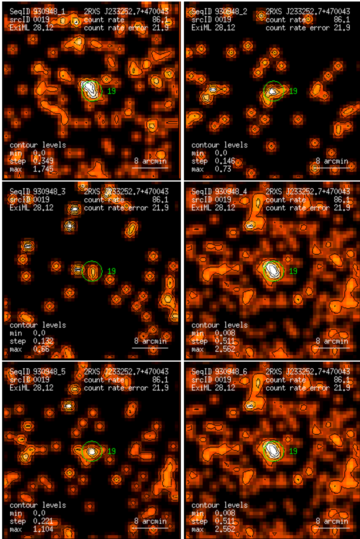
Figure 19: RASS 930948: detection 0019: band rate images, Gaussian filter: (1) PSPC channels 11 – 41, (2) 52 – 90, (3) 91 – 201, (4) 11 – 235, (5) 52 – 201, (6) 11 – 201. Broad band rates in counts/ks. Band rate contour levels in counts/ks/arcmin 2 .
