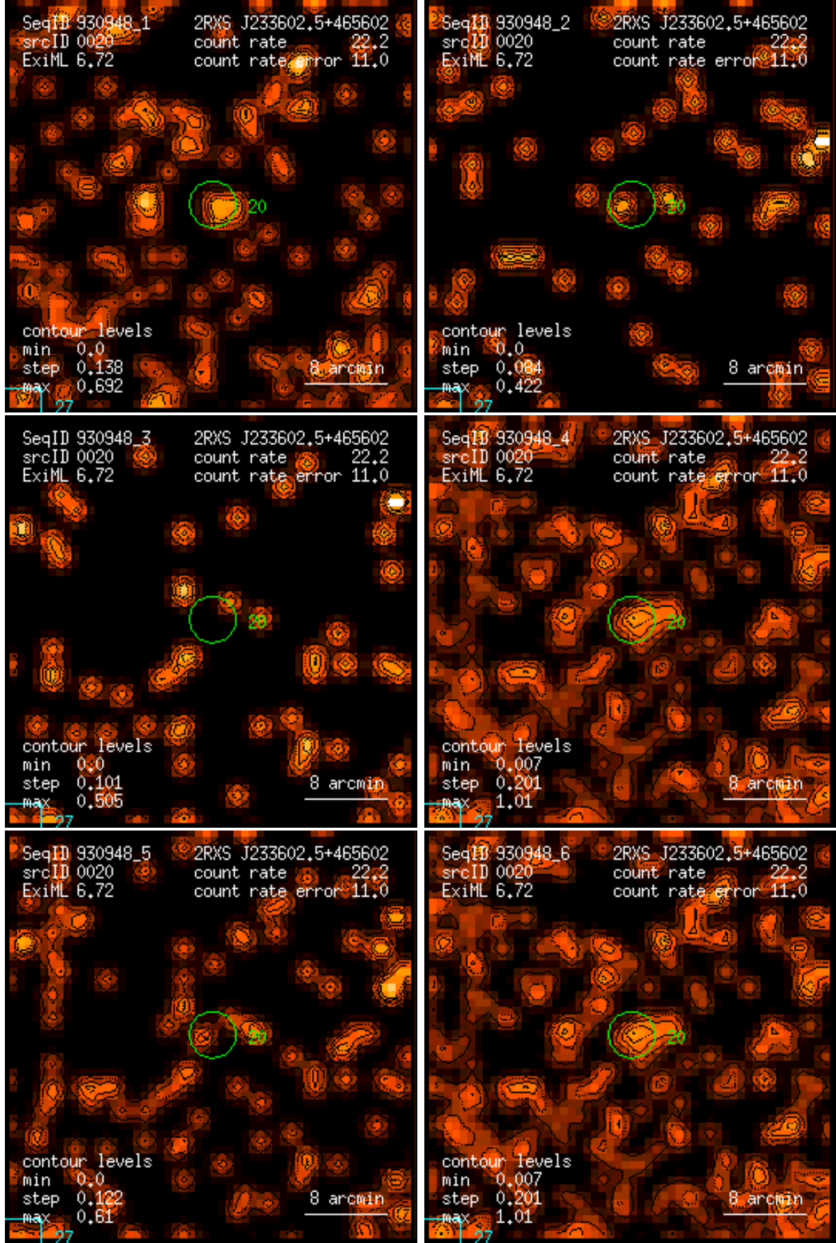
Figure 20: RASS 930948: detection 0020: band rate images, Gaussian filter: (1) PSPC channels 11 – 41, (2) 52 – 90, (3) 91 – 201, (4) 11 – 235, (5) 52 – 201, (6) 11 – 201. Broad band rates in counts/ks. Band rate contour levels in counts/ks/arcmin 2 .
