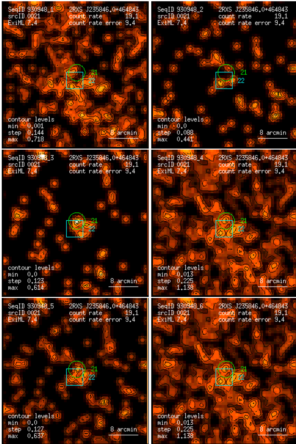
Figure 21: RASS 930948: detection 0021: band rate images, Gaussian filter: (1) PSPC channels 11 – 41, (2) 52 – 90, (3) 91 – 201, (4) 11 – 235, (5) 52 – 201, (6) 11 – 201. Broad band rates in counts/ks. Band rate contour levels in counts/ks/arcmin 2 .
