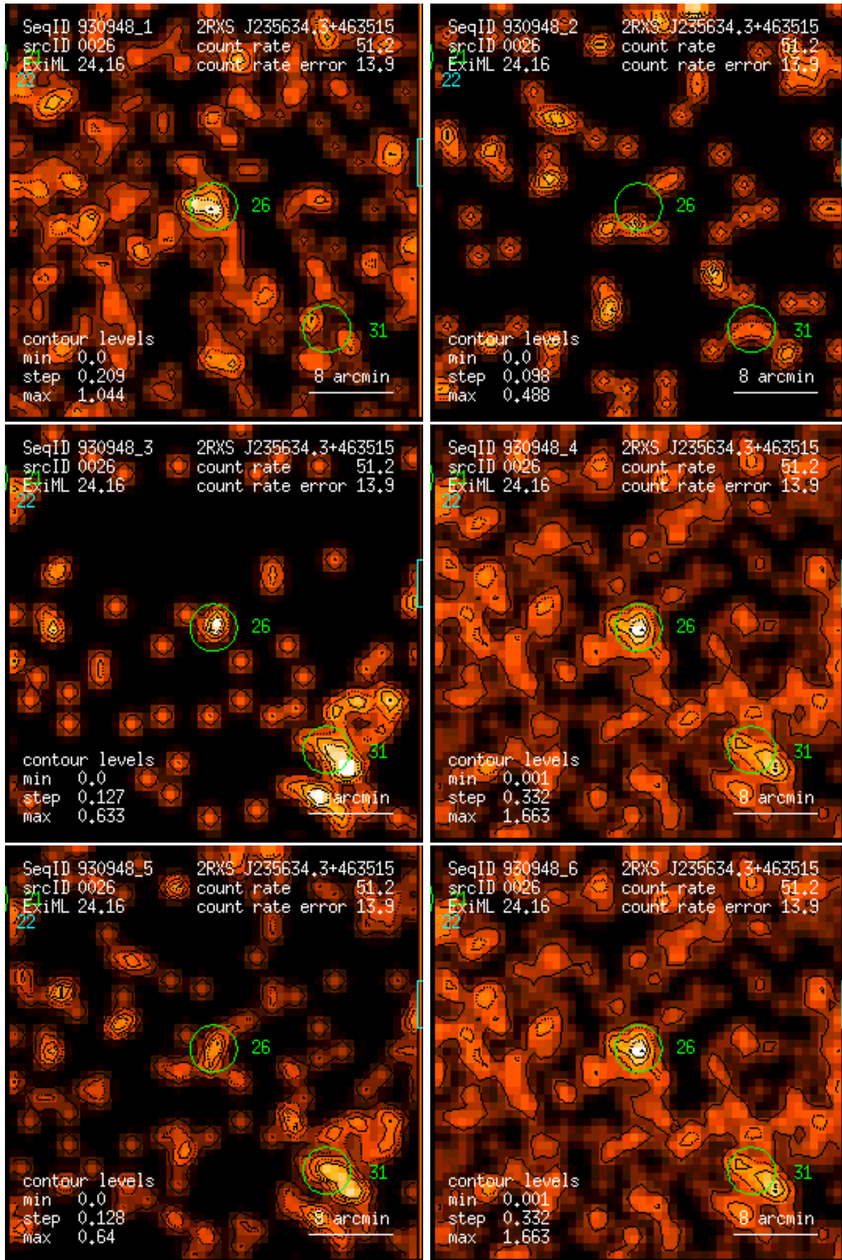
Figure 26: RASS 930948: detection 0026: band rate images, Gaussian filter: (1) PSPC channels 11 – 41, (2) 52 – 90, (3) 91 – 201, (4) 11 – 235, (5) 52 – 201, (6) 11 – 201. Broad band rates in counts/ks. Band rate contour levels in counts/ks/arcmin 2 .
