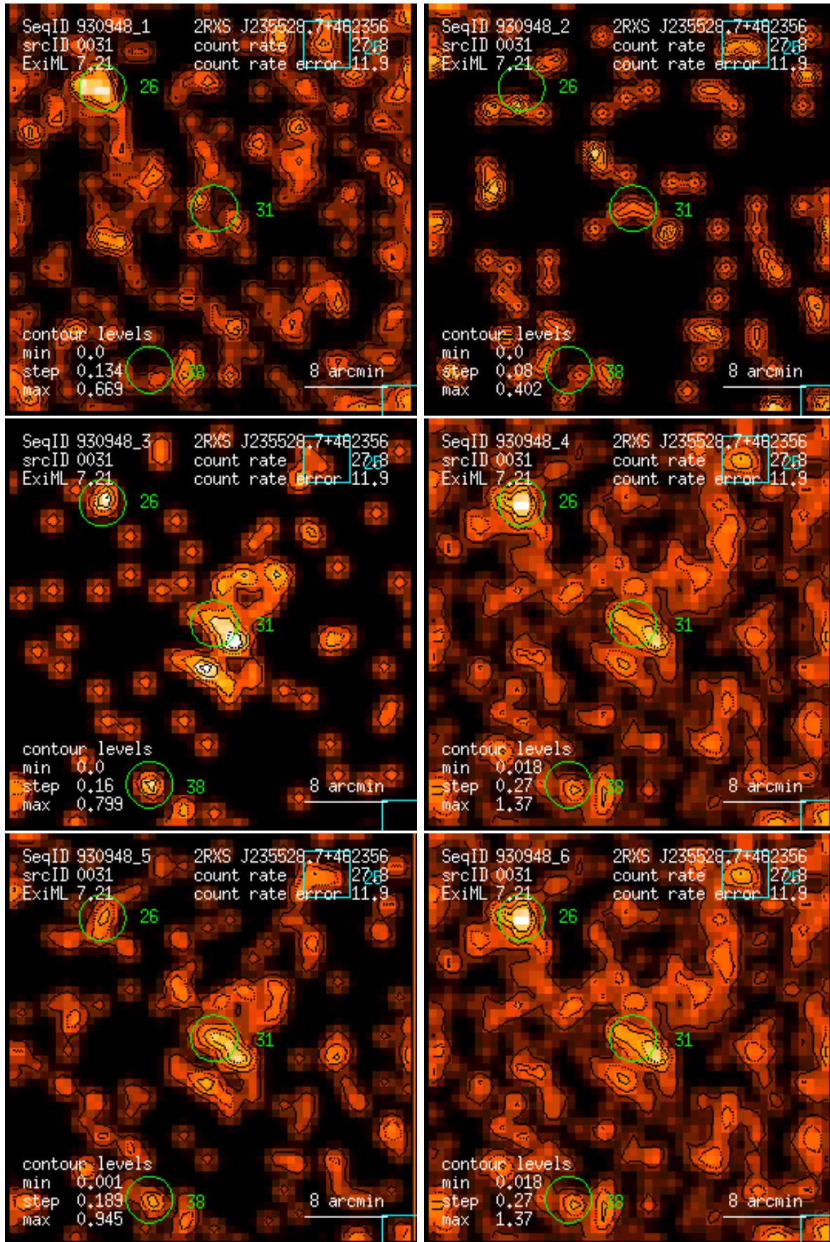
Figure 31: RASS 930948: detection 0031: band rate images, Gaussian filter: (1) PSPC channels 11 – 41, (2) 52 – 90, (3) 91 – 201, (4) 11 – 235, (5) 52 – 201, (6) 11 – 201. Broad band rates in counts/ks. Band rate contour levels in counts/ks/arcmin 2 .
