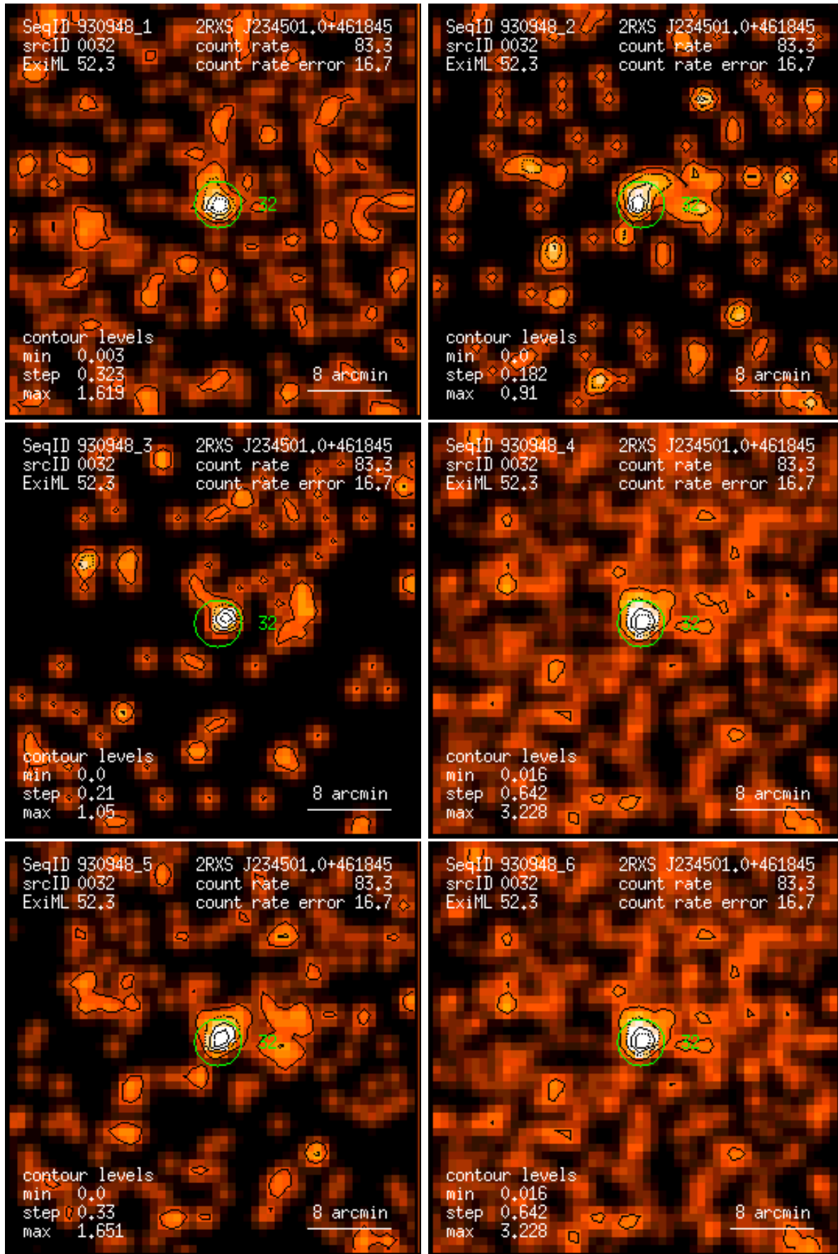
Figure 32: RASS 930948: detection 0032: band rate images, Gaussian filter: (1) PSPC channels 11 – 41, (2) 52 – 90, (3) 91 – 201, (4) 11 – 235, (5) 52 – 201, (6) 11 – 201. Broad band rates in counts/ks. Band rate contour levels in counts/ks/arcmin 2 .
