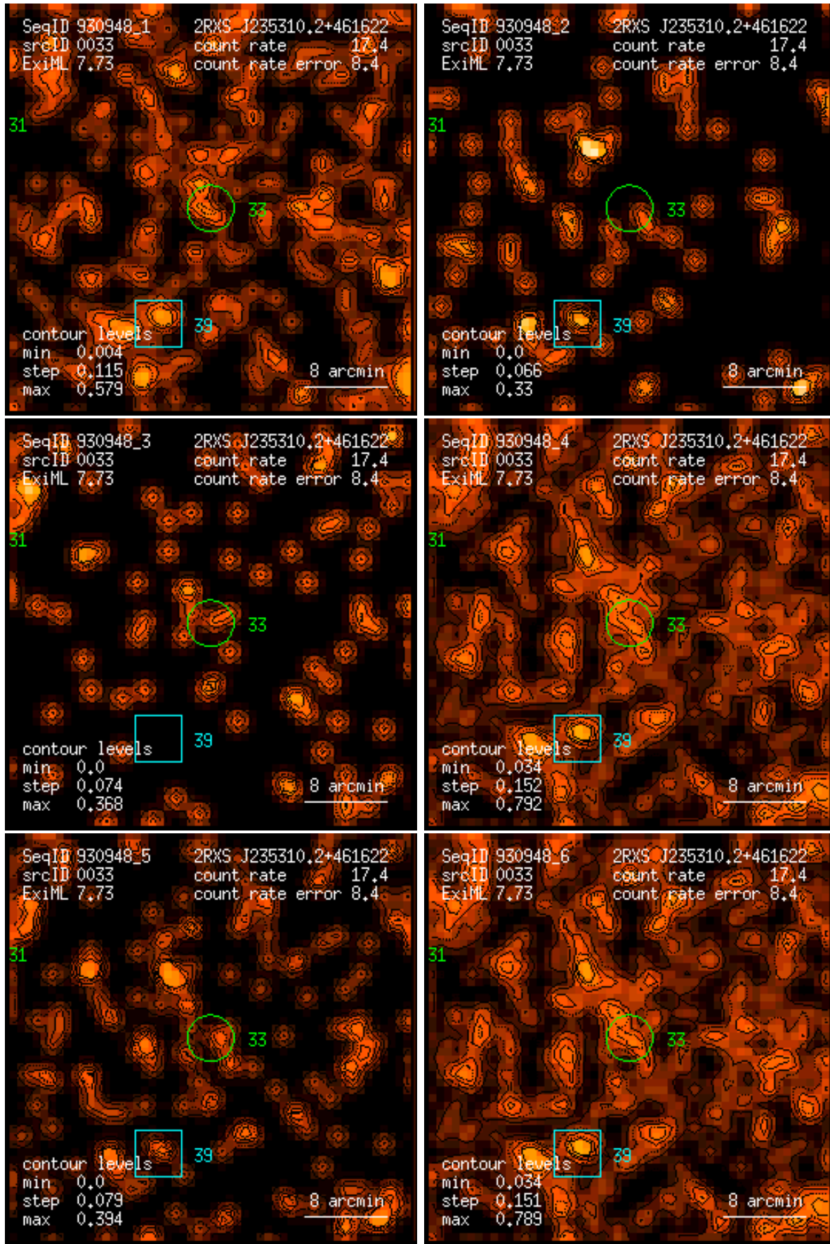
Figure 33: RASS 930948: detection 0033: band rate images, Gaussian filter: (1) PSPC channels 11 – 41, (2) 52 – 90, (3) 91 – 201, (4) 11 – 235, (5) 52 – 201, (6) 11 – 201. Broad band rates in counts/ks. Band rate contour levels in counts/ks/arcmin 2 .
