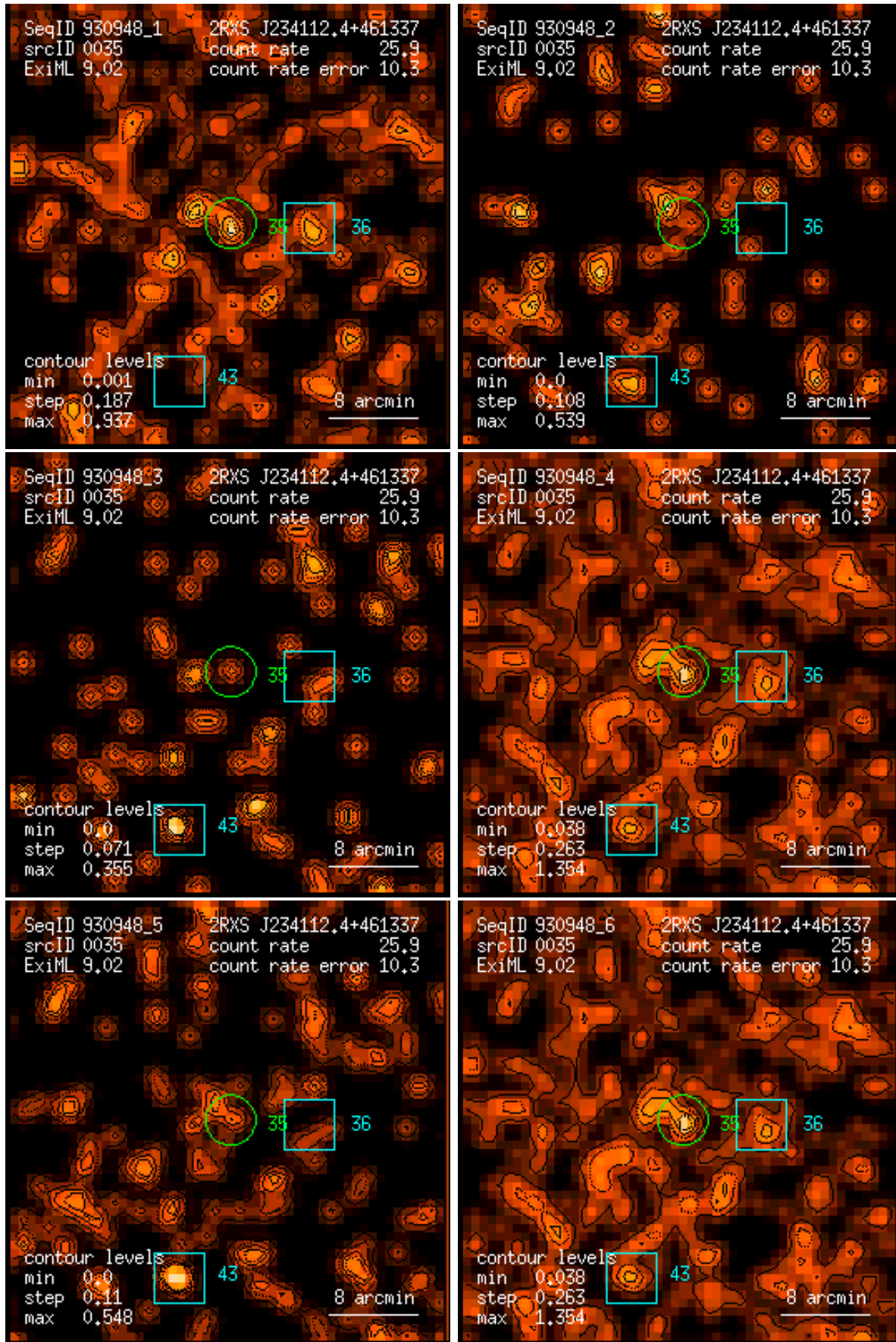
Figure 35: RASS 930948: detection 0035: band rate images, Gaussian filter: (1) PSPC channels 11 – 41, (2) 52 – 90, (3) 91 – 201, (4) 11 – 235, (5) 52 – 201, (6) 11 – 201. Broad band rates in counts/ks. Band rate contour levels in counts/ks/arcmin 2 .
