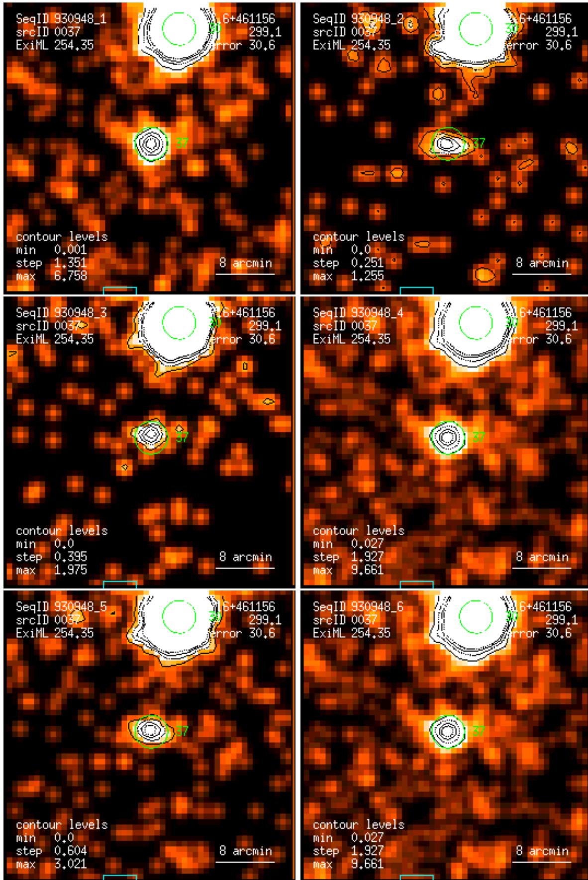
Figure 37: RASS 930948: detection 0037: band rate images, Gaussian filter: (1) PSPC channels 11 – 41, (2) 52 – 90, (3) 91 – 201, (4) 11 – 235, (5) 52 – 201, (6) 11 – 201. Broad band rates in counts/ks. Band rate contour levels in counts/ks/arcmin 2 .
