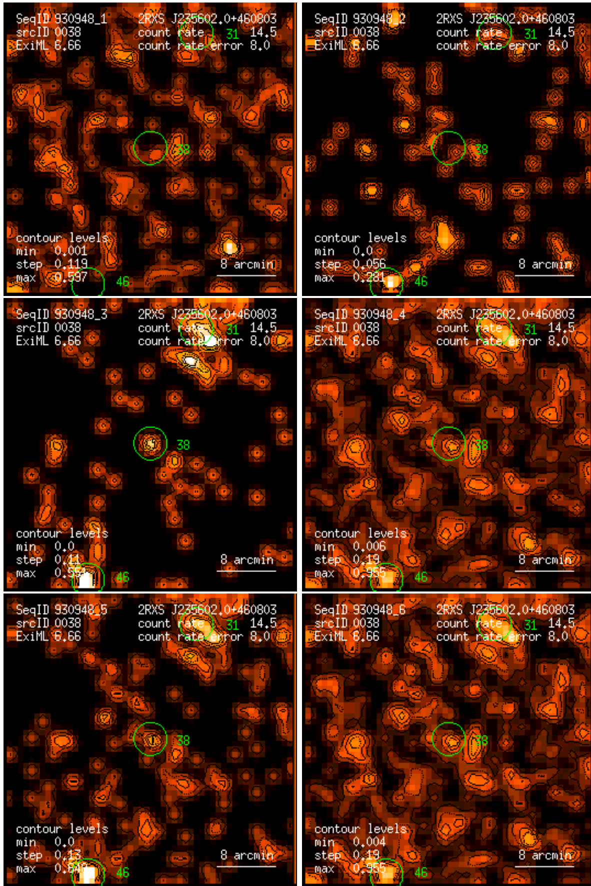
Figure 38: RASS 930948: detection 0038: band rate images, Gaussian filter: (1) PSPC channels 11 – 41, (2) 52 – 90, (3) 91 – 201, (4) 11 – 235, (5) 52 – 201, (6) 11 – 201. Broad band rates in counts/ks. Band rate contour levels in counts/ks/arcmin 2 .
