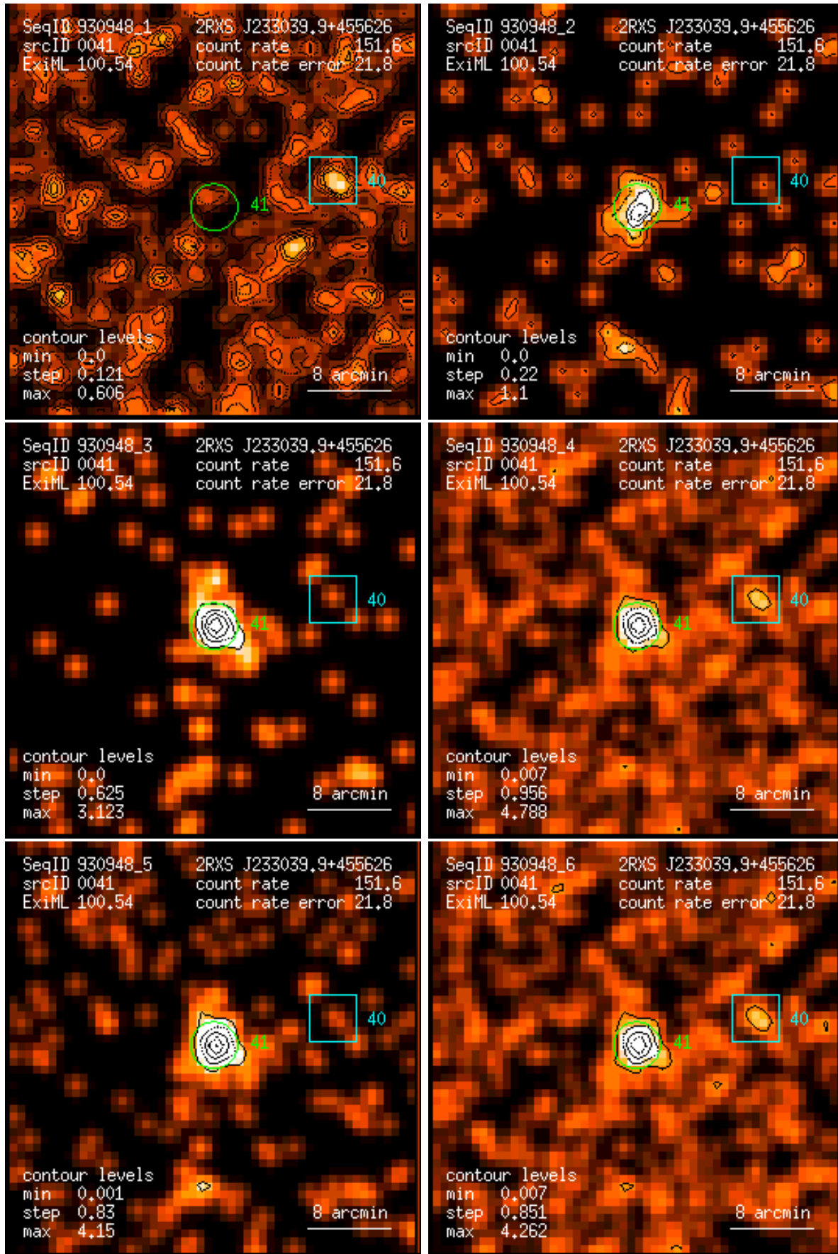
Figure 41: RASS 930948: detection 0041: band rate images, Gaussian filter: (1) PSPC channels 11 – 41, (2) 52 – 90, (3) 91 – 201, (4) 11 – 235, (5) 52 – 201, (6) 11 – 201. Broad band rates in counts/ks. Band rate contour levels in counts/ks/arcmin 2 .
