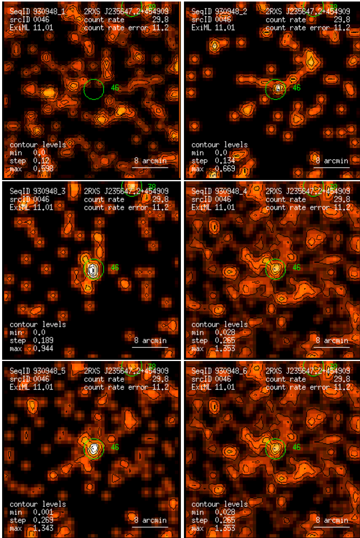
Figure 46: RASS 930948: detection 0046: band rate images, Gaussian filter: (1) PSPC channels 11 – 41, (2) 52 – 90, (3) 91 – 201, (4) 11 – 235, (5) 52 – 201, (6) 11 – 201. Broad band rates in counts/ks. Band rate contour levels in counts/ks/arcmin 2 .
