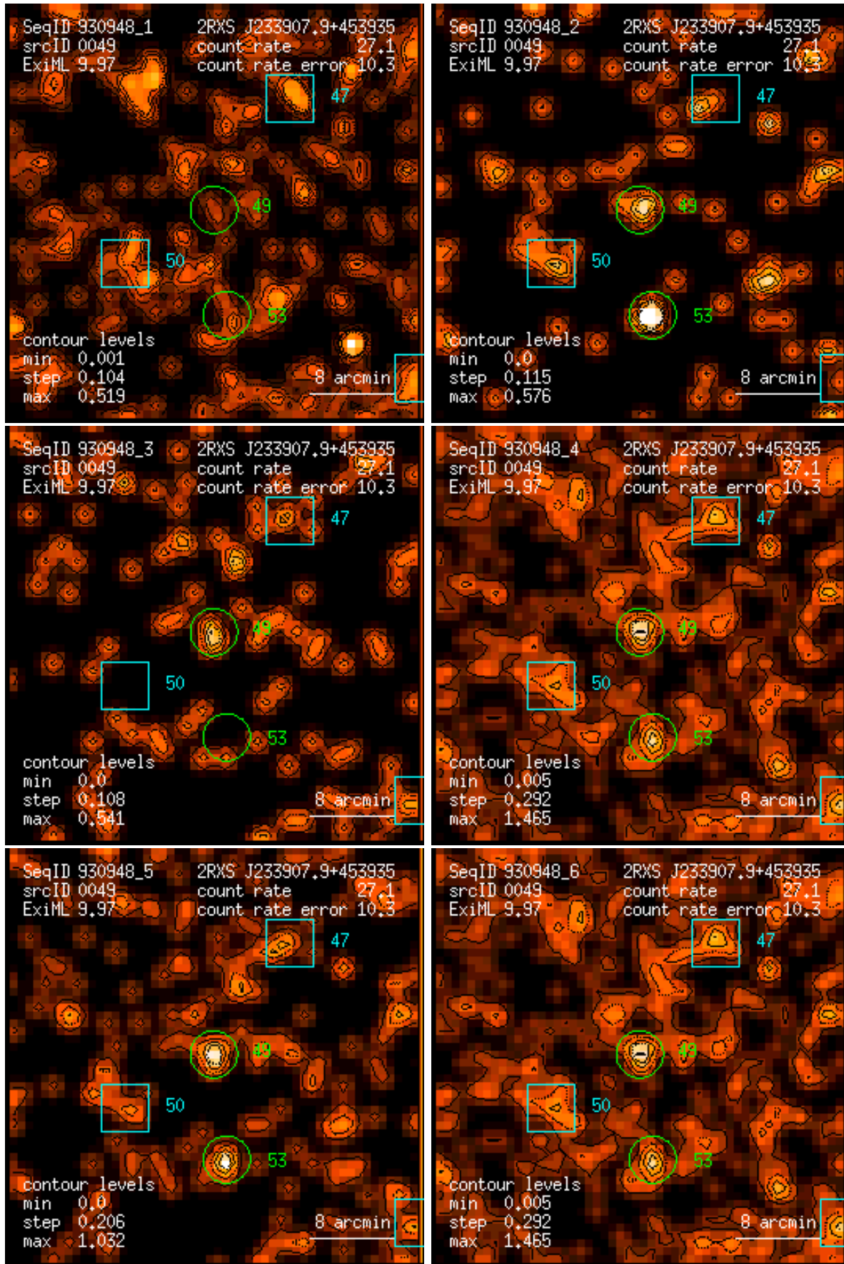
Figure 49: RASS 930948: detection 0049: band rate images, Gaussian filter: (1) PSPC channels 11 – 41, (2) 52 – 90, (3) 91 – 201, (4) 11 – 235, (5) 52 – 201, (6) 11 – 201. Broad band rates in counts/ks. Band rate contour levels in counts/ks/arcmin 2 .
