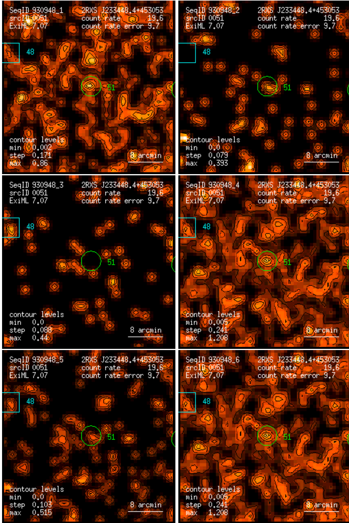
Figure 51: RASS 930948: detection 0051: band rate images, Gaussian filter: (1) PSPC channels 11 – 41, (2) 52 – 90, (3) 91 – 201, (4) 11 – 235, (5) 52 – 201, (6) 11 – 201. Broad band rates in counts/ks. Band rate contour levels in counts/ks/arcmin 2 .
