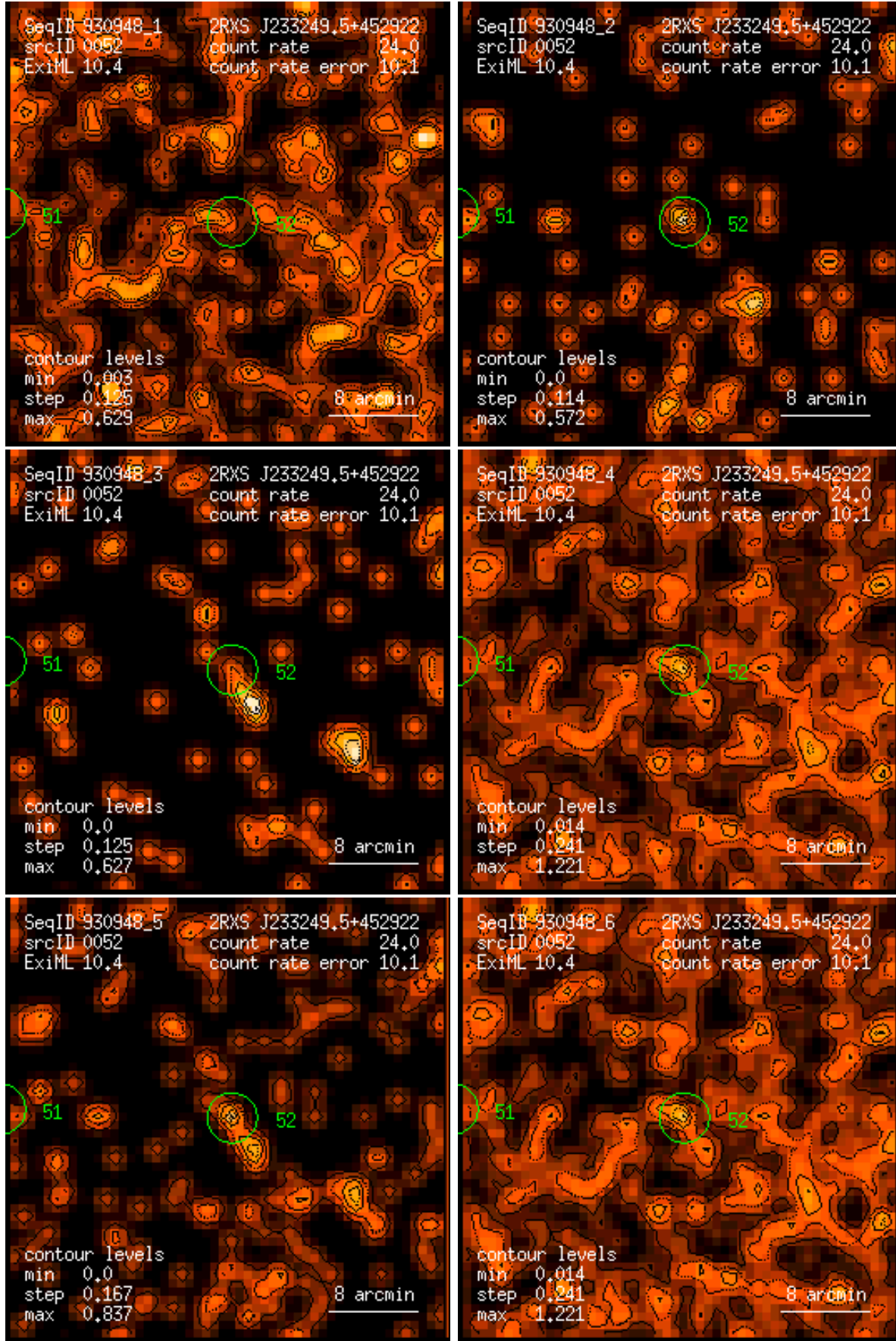
Figure 52: RASS 930948: detection 0052: band rate images, Gaussian filter: (1) PSPC channels 11 – 41, (2) 52 – 90, (3) 91 – 201, (4) 11 – 235, (5) 52 – 201, (6) 11 – 201. Broad band rates in counts/ks. Band rate contour levels in counts/ks/arcmin 2 .
