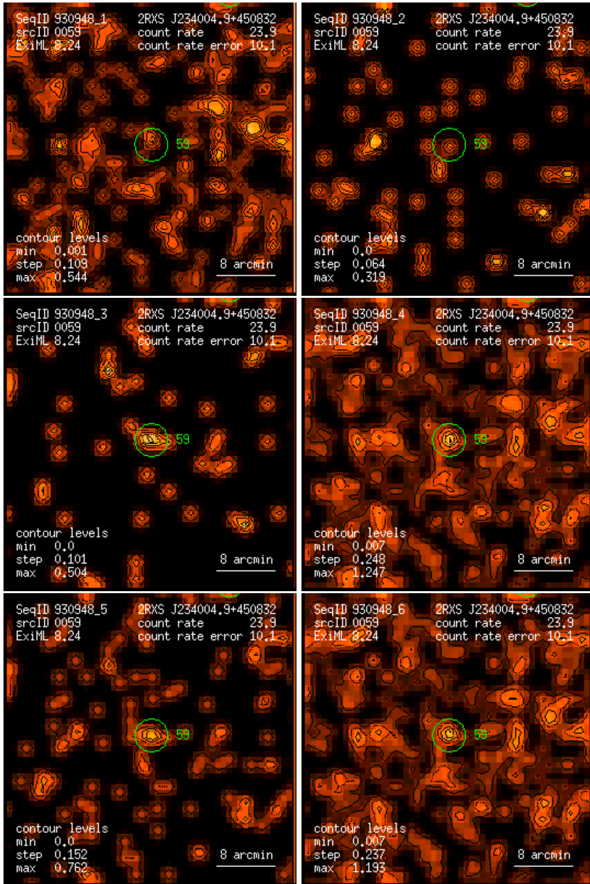
Figure 59: RASS 930948: detection 0059: band rate images, Gaussian filter: (1) PSPC channels 11 – 41, (2) 52 – 90, (3) 91 – 201, (4) 11 – 235, (5) 52 – 201, (6) 11 – 201. Broad band rates in counts/ks. Band rate contour levels in counts/ks/arcmin 2 .
