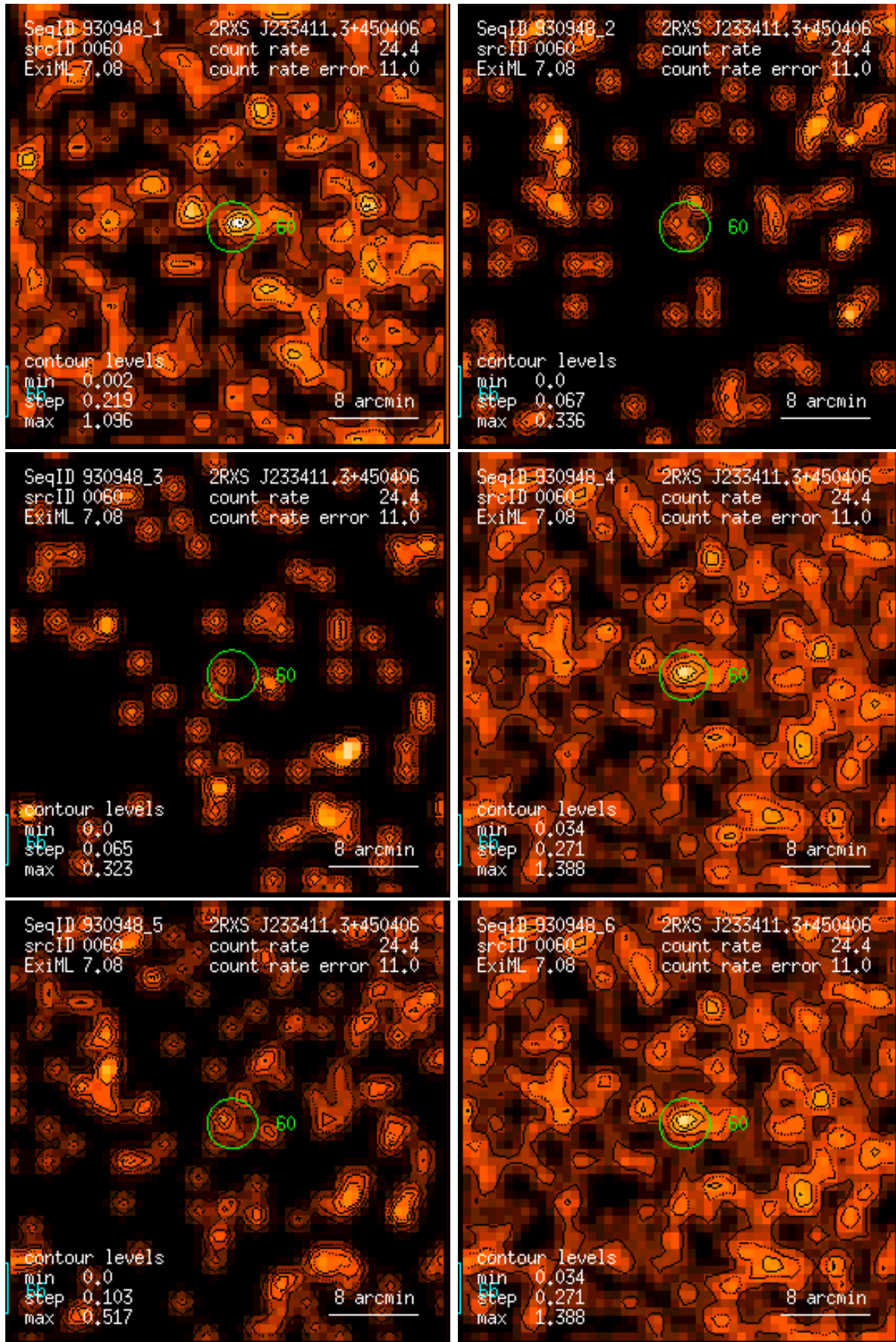
Figure 60: RASS 930948: detection 0060: band rate images, Gaussian filter: (1) PSPC channels 11 – 41, (2) 52 – 90, (3) 91 – 201, (4) 11 – 235, (5) 52 – 201, (6) 11 – 201. Broad band rates in counts/ks. Band rate contour levels in counts/ks/arcmin 2 .
