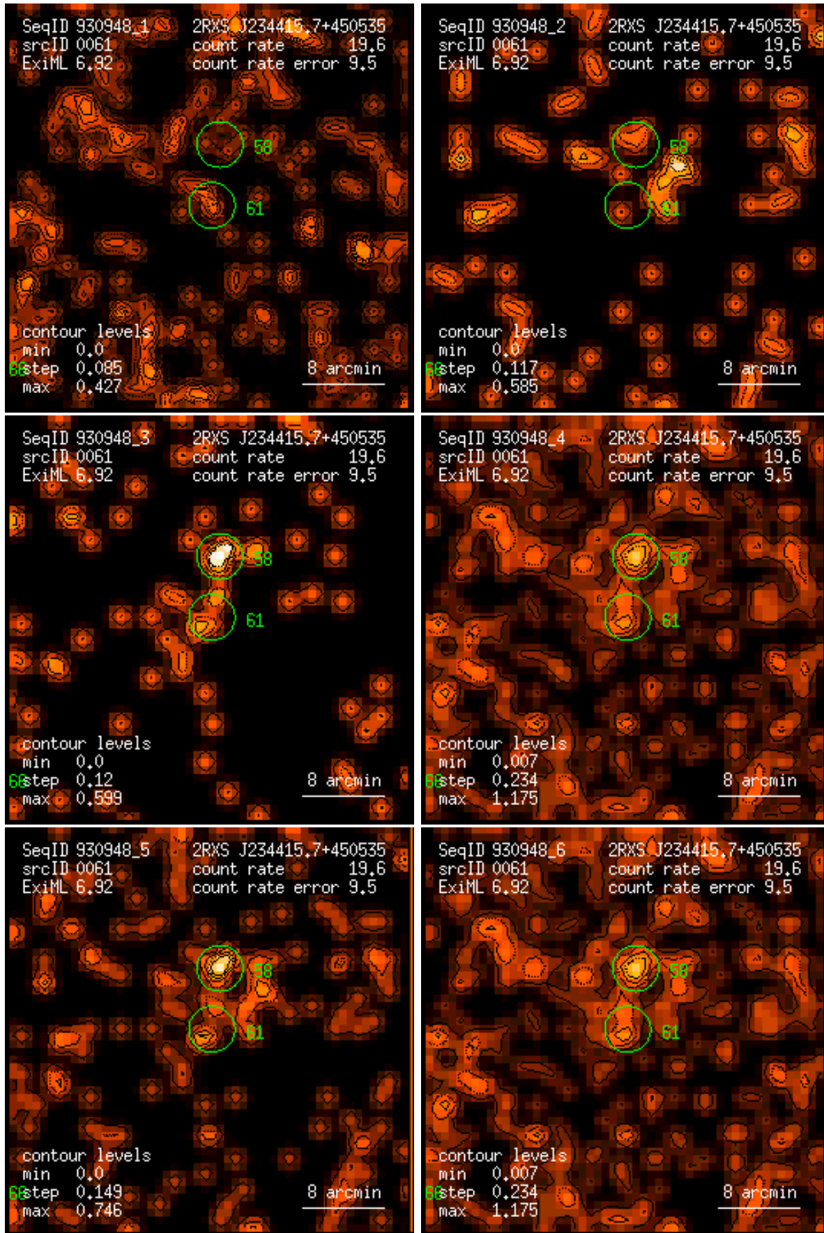
Figure 61: RASS 930948: detection 0061: band rate images, Gaussian filter: (1) PSPC channels 11 – 41, (2) 52 – 90, (3) 91 – 201, (4) 11 – 235, (5) 52 – 201, (6) 11 – 201. Broad band rates in counts/ks. Band rate contour levels in counts/ks/arcmin 2 .
