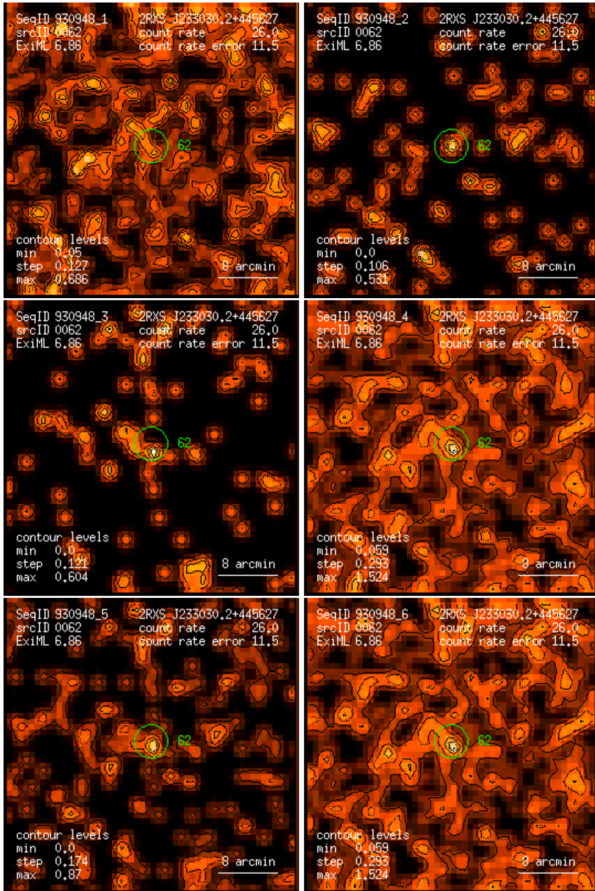
Figure 62: RASS 930948: detection 0062: band rate images, Gaussian filter: (1) PSPC channels 11 – 41, (2) 52 – 90, (3) 91 – 201, (4) 11 – 235, (5) 52 – 201, (6) 11 – 201. Broad band rates in counts/ks. Band rate contour levels in counts/ks/arcmin 2 .
