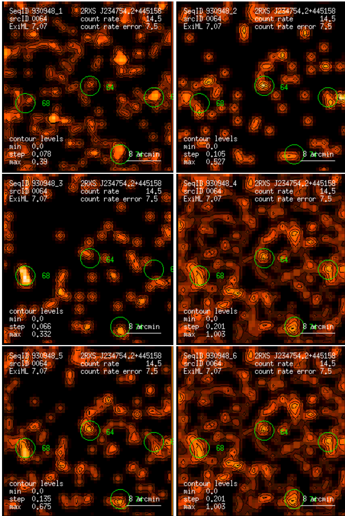
Figure 64: RASS 930948: detection 0064: band rate images, Gaussian filter: (1) PSPC channels 11 – 41, (2) 52 – 90, (3) 91 – 201, (4) 11 – 235, (5) 52 – 201, (6) 11 – 201. Broad band rates in counts/ks. Band rate contour levels in counts/ks/arcmin 2 .
