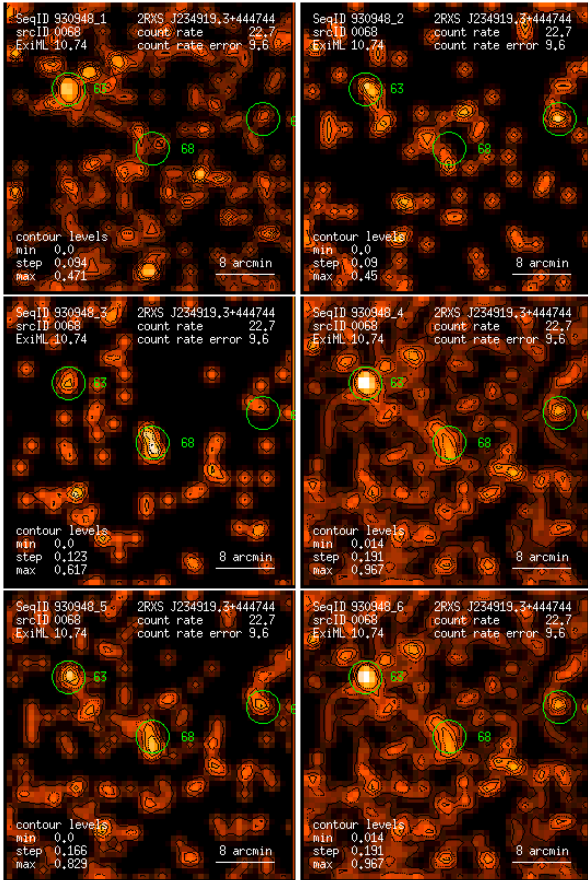
Figure 68: RASS 930948: detection 0068: band rate images, Gaussian filter: (1) PSPC channels 11 – 41, (2) 52 – 90, (3) 91 – 201, (4) 11 – 235, (5) 52 – 201, (6) 11 – 201. Broad band rates in counts/ks. Band rate contour levels in counts/ks/arcmin 2 .
