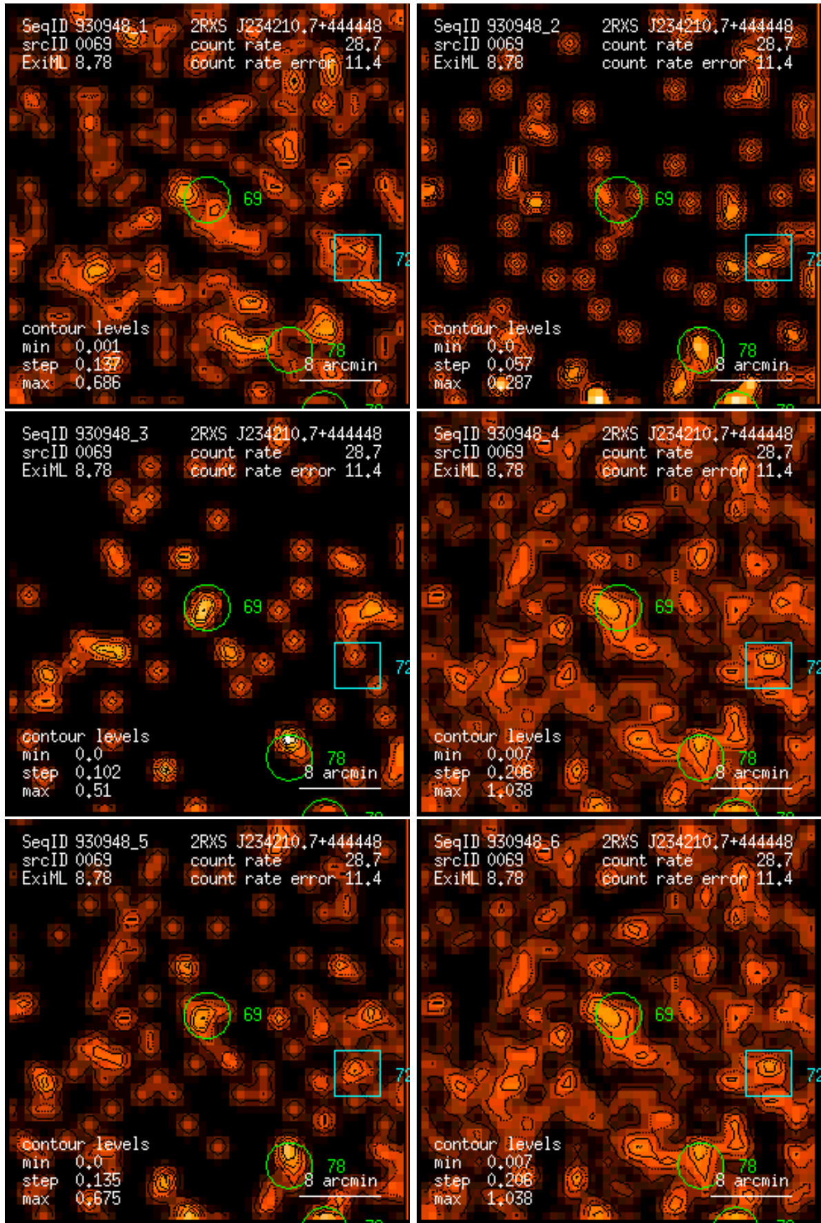
Figure 69: RASS 930948: detection 0069: band rate images, Gaussian filter: (1) PSPC channels 11 – 41, (2) 52 – 90, (3) 91 – 201, (4) 11 – 235, (5) 52 – 201, (6) 11 – 201. Broad band rates in counts/ks. Band rate contour levels in counts/ks/arcmin 2 .
