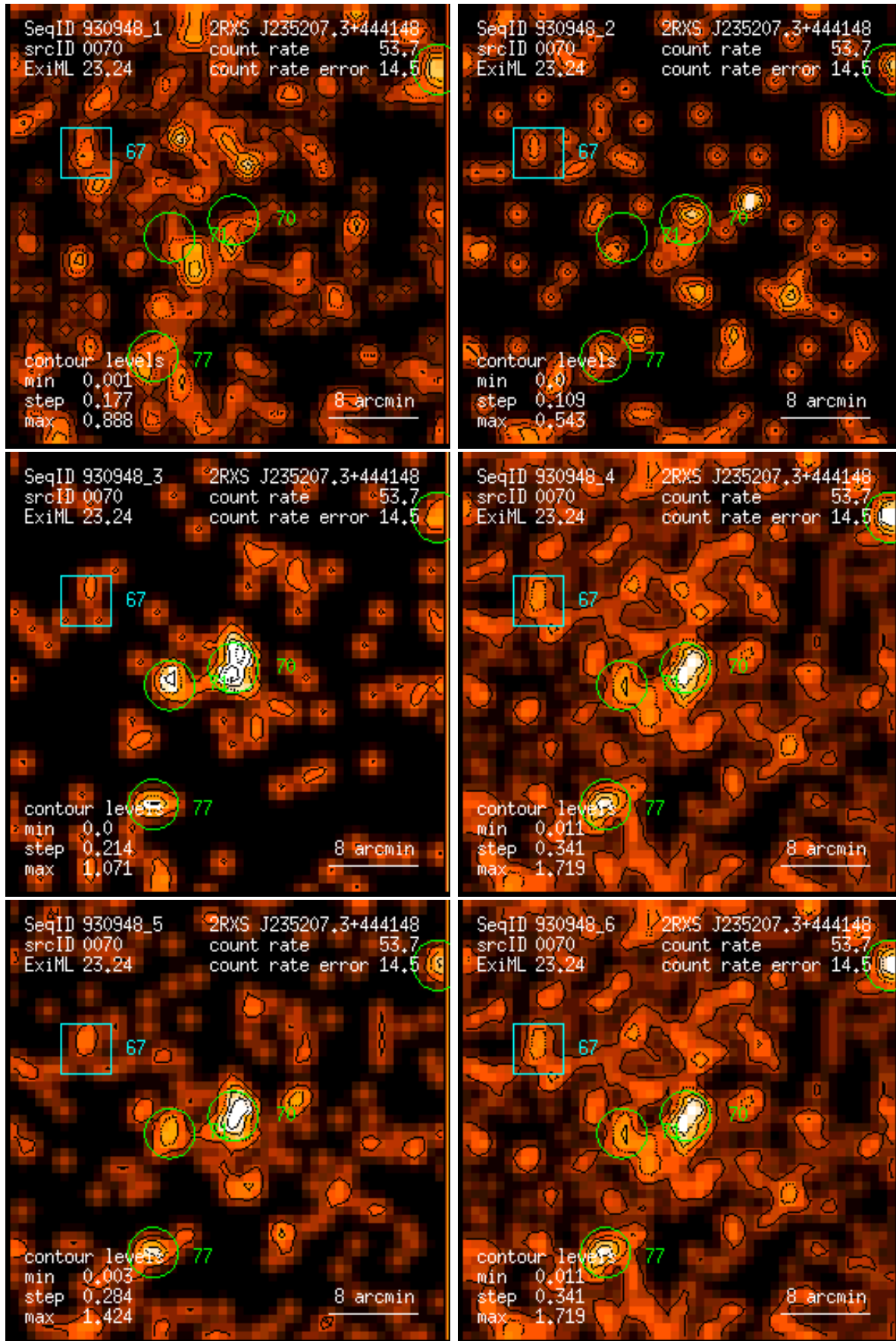
Figure 70: RASS 930948: detection 0070: band rate images, Gaussian filter: (1) PSPC channels 11 – 41, (2) 52 – 90, (3) 91 – 201, (4) 11 – 235, (5) 52 – 201, (6) 11 – 201. Broad band rates in counts/ks. Band rate contour levels in counts/ks/arcmin 2 .
