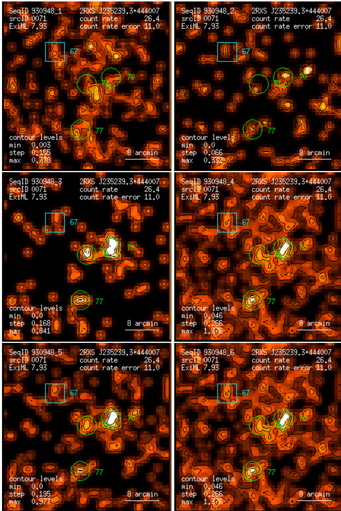
Figure 71: RASS 930948: detection 0071: band rate images, Gaussian filter: (1) PSPC channels 11 – 41, (2) 52 – 90, (3) 91 – 201, (4) 11 – 235, (5) 52 – 201, (6) 11 – 201. Broad band rates in counts/ks. Band rate contour levels in counts/ks/arcmin 2 .
