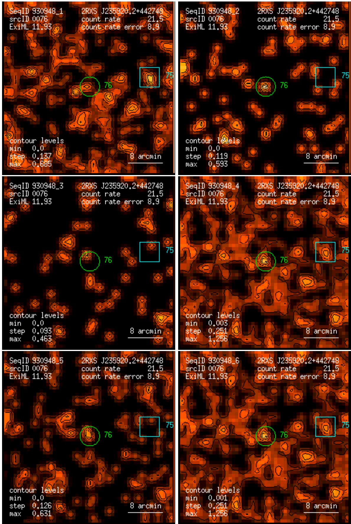
Figure 76: RASS 930948: detection 0076: band rate images, Gaussian filter: (1) PSPC channels 11 – 41, (2) 52 – 90, (3) 91 – 201, (4) 11 – 235, (5) 52 – 201, (6) 11 – 201. Broad band rates in counts/ks. Band rate contour levels in counts/ks/arcmin 2 .
