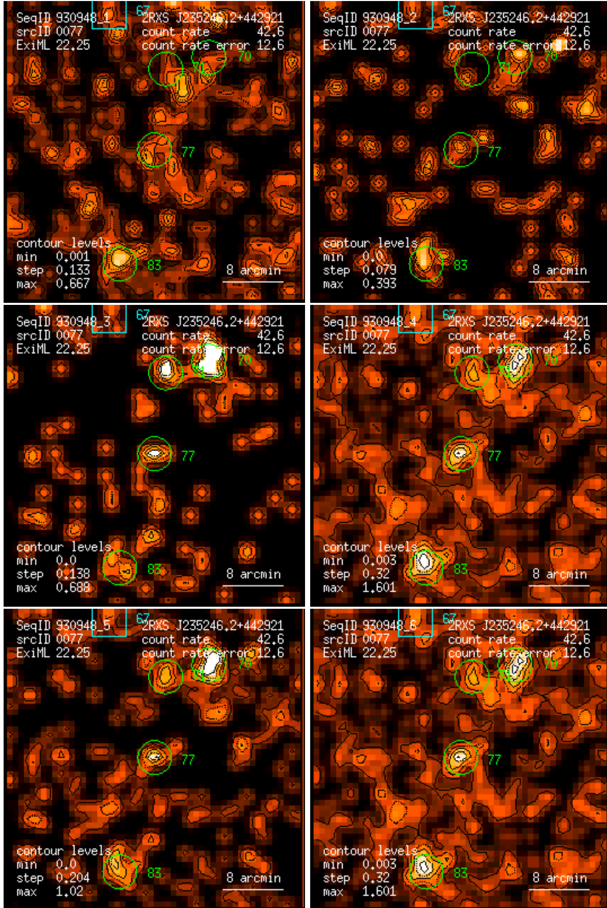
Figure 77: RASS 930948: detection 0077: band rate images, Gaussian filter: (1) PSPC channels 11 – 41, (2) 52 – 90, (3) 91 – 201, (4) 11 – 235, (5) 52 – 201, (6) 11 – 201. Broad band rates in counts/ks. Band rate contour levels in counts/ks/arcmin 2 .
