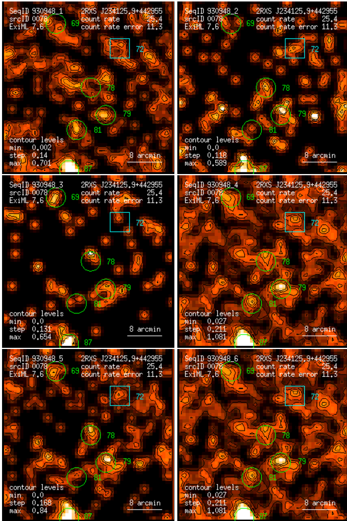
Figure 78: RASS 930948: detection 0078: band rate images, Gaussian filter: (1) PSPC channels 11 – 41, (2) 52 – 90, (3) 91 – 201, (4) 11 – 235, (5) 52 – 201, (6) 11 – 201. Broad band rates in counts/ks. Band rate contour levels in counts/ks/arcmin 2 .
