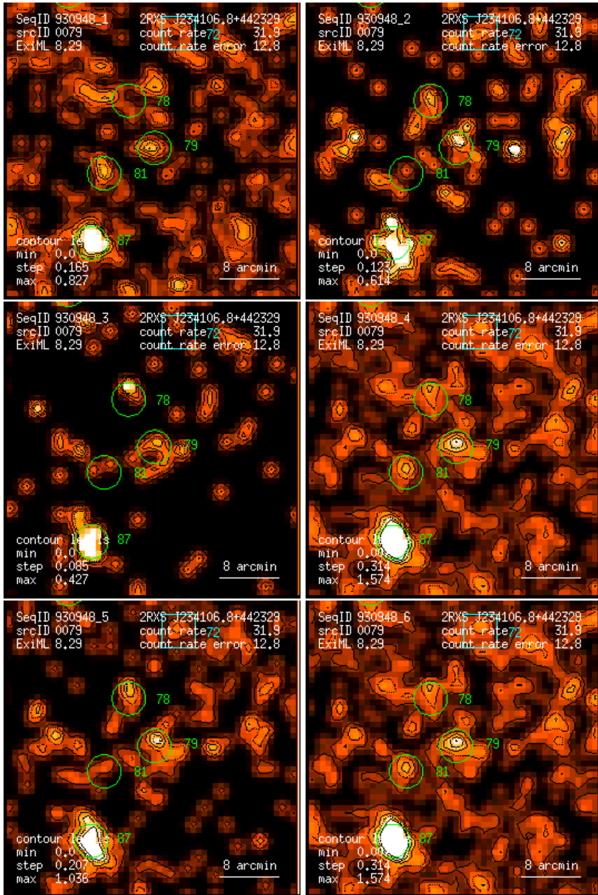
Figure 79: RASS 930948: detection 0079: band rate images, Gaussian filter: (1) PSPC channels 11 – 41, (2) 52 – 90, (3) 91 – 201, (4) 11 – 235, (5) 52 – 201, (6) 11 – 201. Broad band rates in counts/ks. Band rate contour levels in counts/ks/arcmin 2 .
