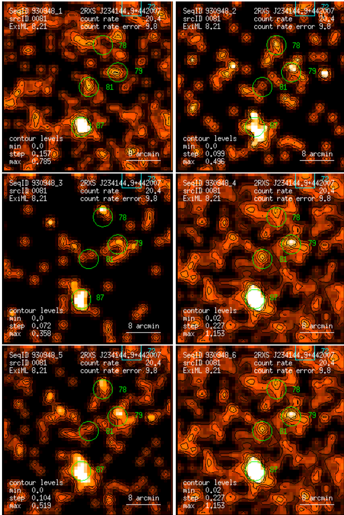
Figure 81: RASS 930948: detection 0081: band rate images, Gaussian filter: (1) PSPC channels 11 – 41, (2) 52 – 90, (3) 91 – 201, (4) 11 – 235, (5) 52 – 201, (6) 11 – 201. Broad band rates in counts/ks. Band rate contour levels in counts/ks/arcmin 2 .
