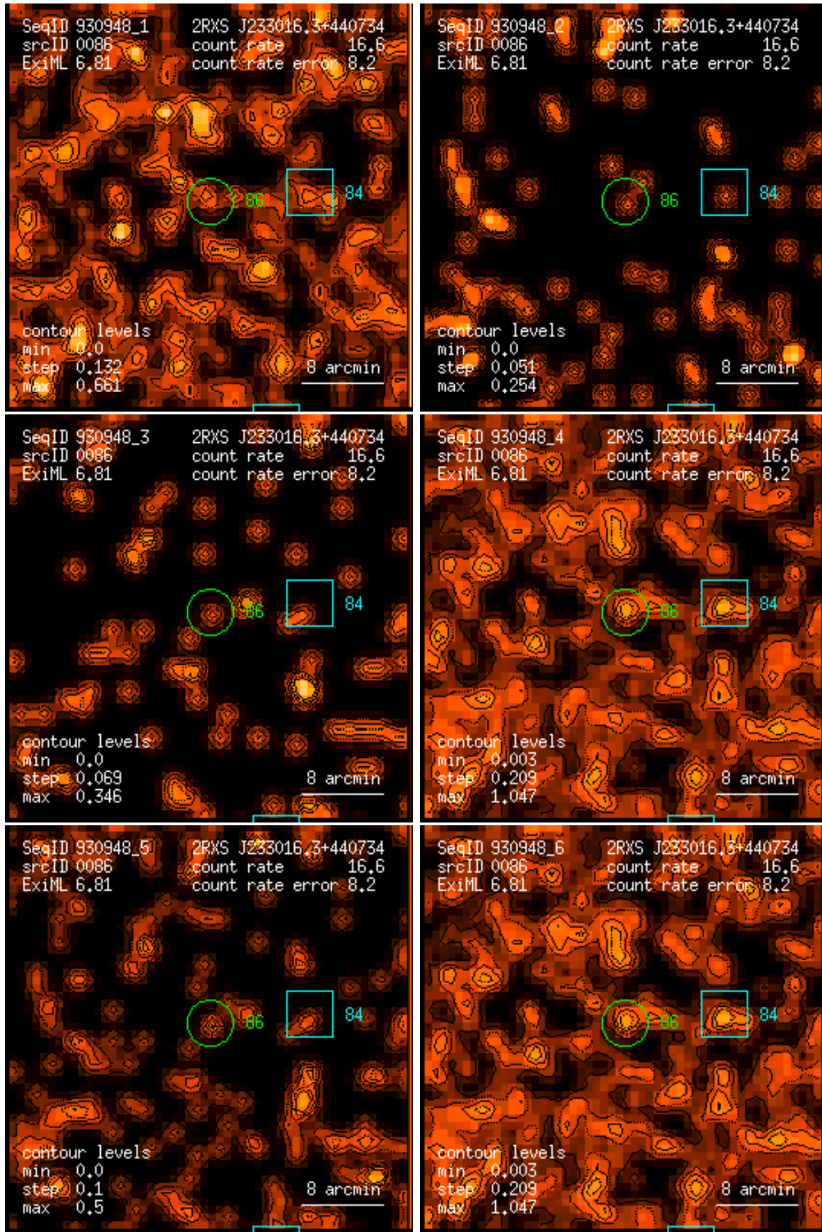
Figure 86: RASS 930948: detection 0086: band rate images, Gaussian filter: (1) PSPC channels 11 – 41, (2) 52 – 90, (3) 91 – 201, (4) 11 – 235, (5) 52 – 201, (6) 11 – 201. Broad band rates in counts/ks. Band rate contour levels in counts/ks/arcmin 2 .
