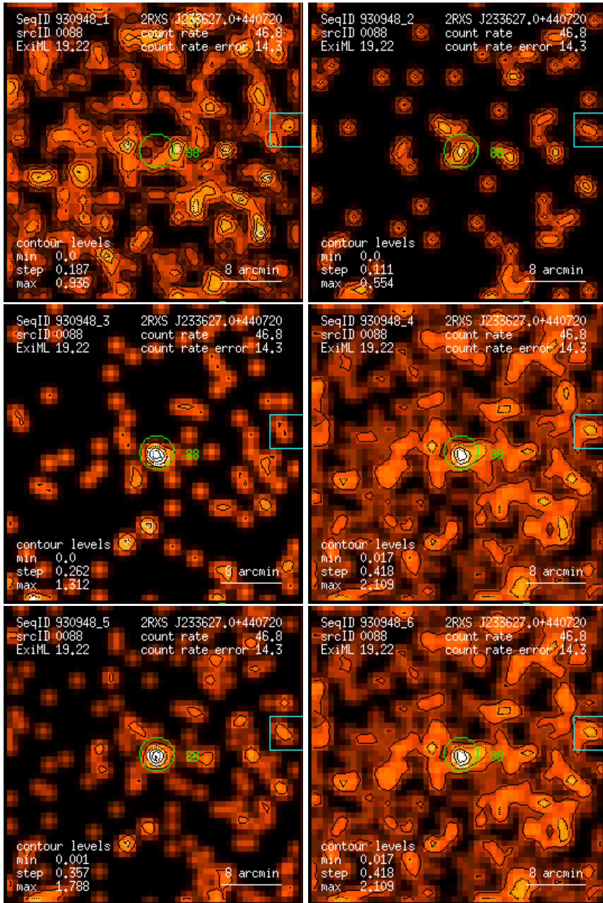
Figure 88: RASS 930948: detection 0088: band rate images, Gaussian filter: (1) PSPC channels 11 – 41, (2) 52 – 90, (3) 91 – 201, (4) 11 – 235, (5) 52 – 201, (6) 11 – 201. Broad band rates in counts/ks. Band rate contour levels in counts/ks/arcmin 2 .
