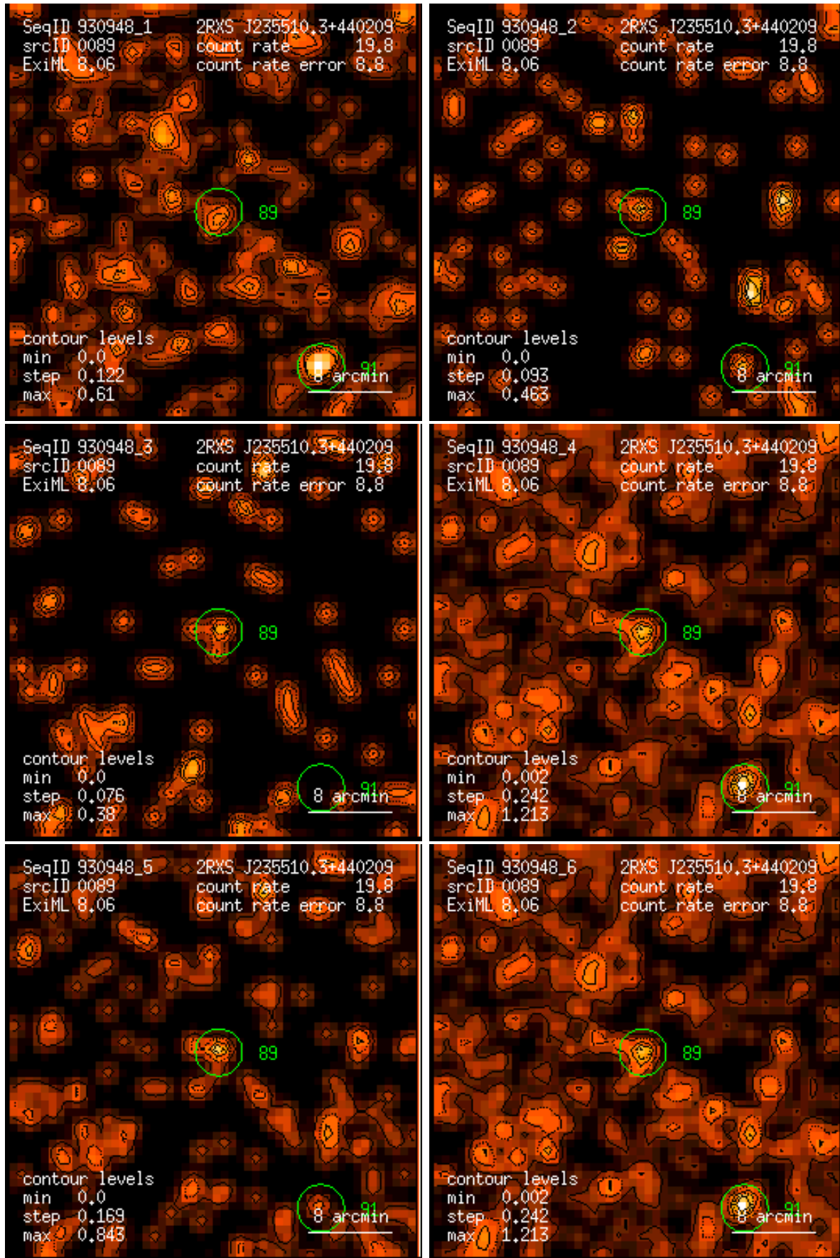
Figure 89: RASS 930948: detection 0089: band rate images, Gaussian filter: (1) PSPC channels 11 – 41, (2) 52 – 90, (3) 91 – 201, (4) 11 – 235, (5) 52 – 201, (6) 11 – 201. Broad band rates in counts/ks. Band rate contour levels in counts/ks/arcmin 2 .
