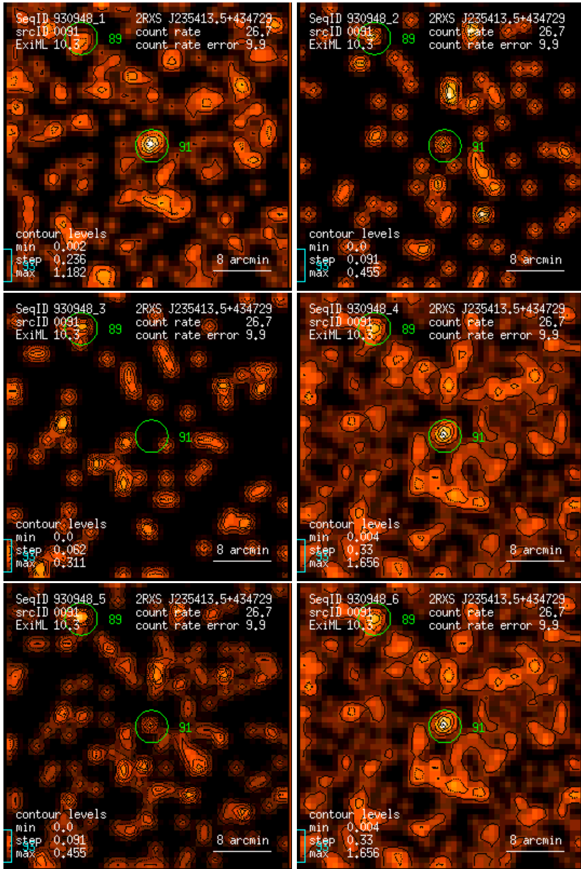
Figure 91: RASS 930948: detection 0091: band rate images, Gaussian filter: (1) PSPC channels 11 – 41, (2) 52 – 90, (3) 91 – 201, (4) 11 – 235, (5) 52 – 201, (6) 11 – 201. Broad band rates in counts/ks. Band rate contour levels in counts/ks/arcmin 2 .
