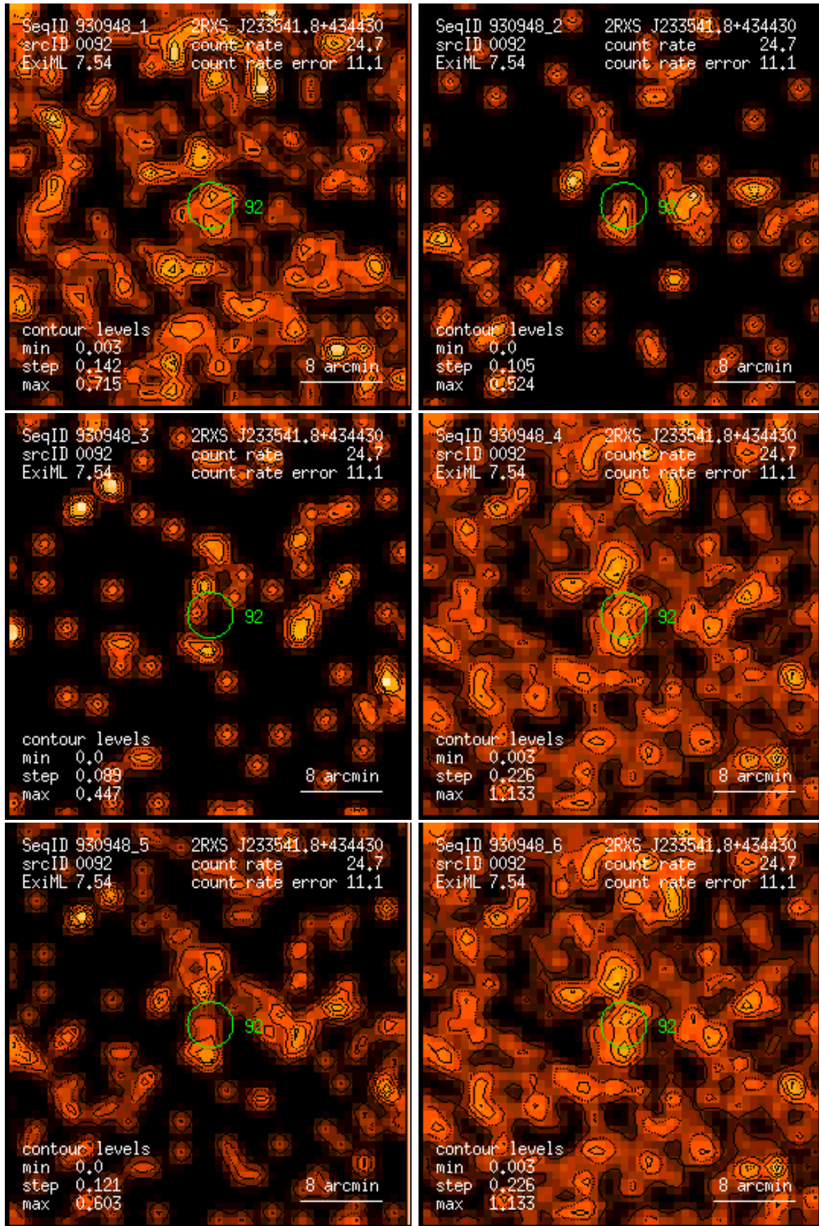
Figure 92: RASS 930948: detection 0092: band rate images, Gaussian filter: (1) PSPC channels 11 – 41, (2) 52 – 90, (3) 91 – 201, (4) 11 – 235, (5) 52 – 201, (6) 11 – 201. Broad band rates in counts/ks. Band rate contour levels in counts/ks/arcmin 2 .
