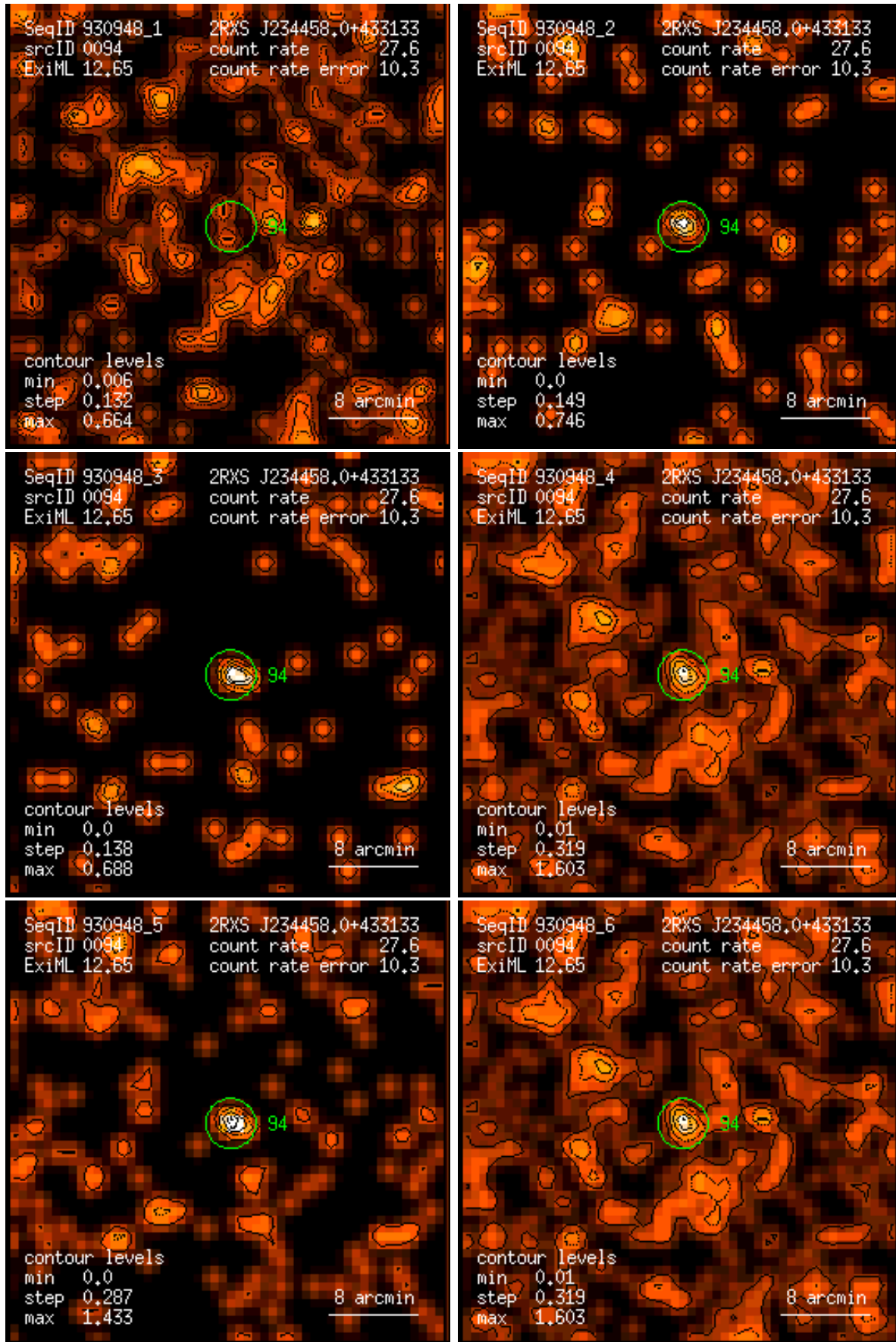
Figure 94: RASS 930948: detection 0094: band rate images, Gaussian filter: (1) PSPC channels 11 – 41, (2) 52 – 90, (3) 91 – 201, (4) 11 – 235, (5) 52 – 201, (6) 11 – 201. Broad band rates in counts/ks. Band rate contour levels in counts/ks/arcmin 2 .
