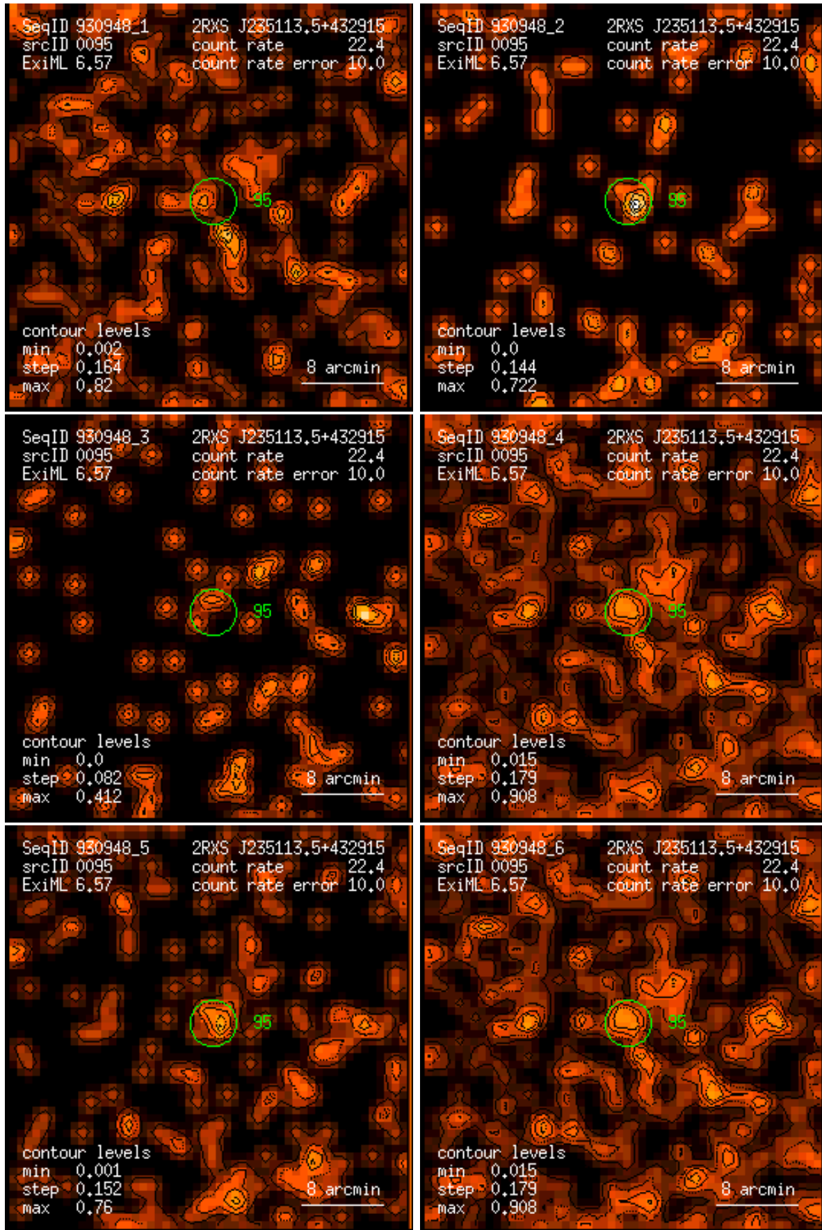
Figure 95: RASS 930948: detection 0095: band rate images, Gaussian filter: (1) PSPC channels 11 – 41, (2) 52 – 90, (3) 91 – 201, (4) 11 – 235, (5) 52 – 201, (6) 11 – 201. Broad band rates in counts/ks. Band rate contour levels in counts/ks/arcmin 2 .
